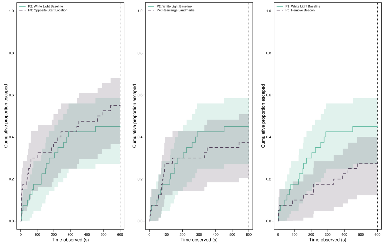
Figure 6: P2 vs. P3/P4/P5: Time survival curves (3 panels)
