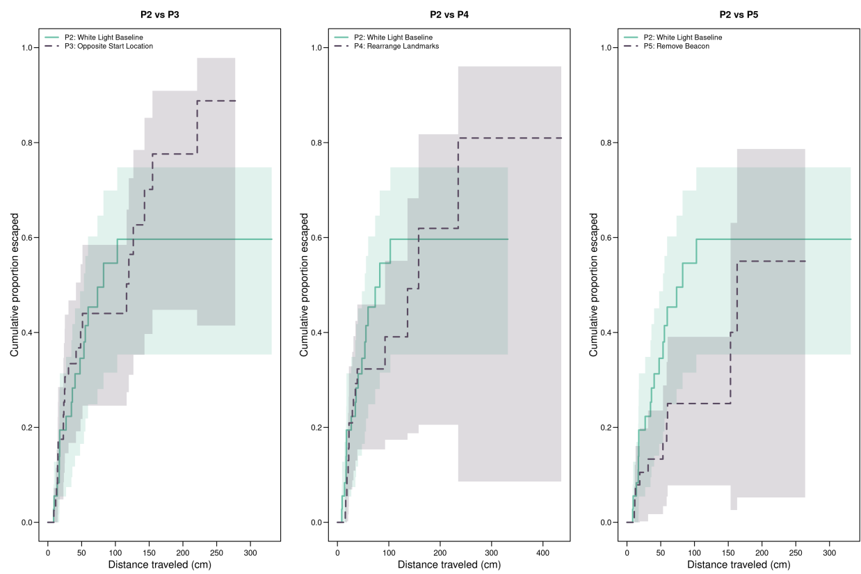
Figure 7: P2 vs. P3/P4/P5: Distance survival curves (3 panels)
