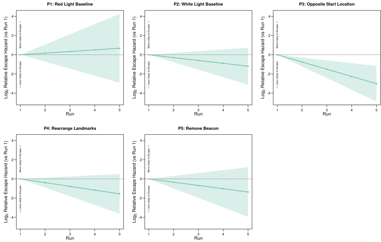
Figure 1: Within-trial Cox: log-relative hazard by run — time (5 panels)
