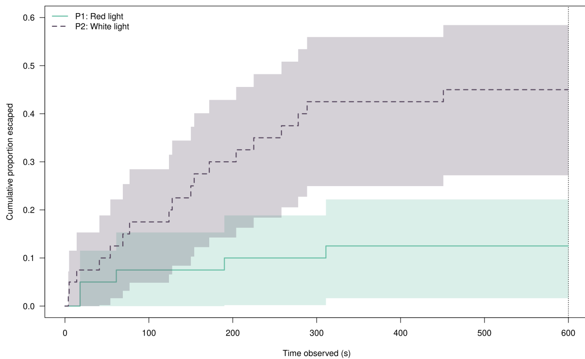
Figure 4: P1 vs. P2: Cumulative proportion escaped with 95% CI
