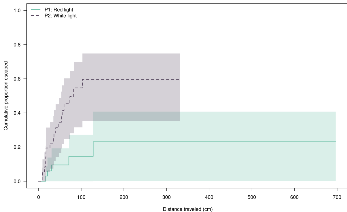
Figure 5: P1 vs. P2: Distance survival with 95% CI
