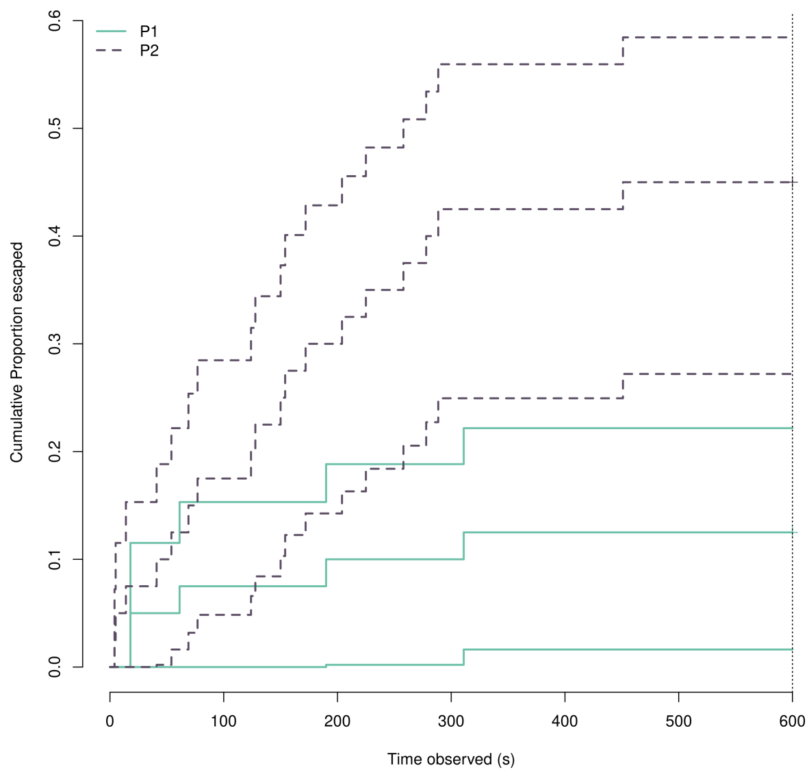
Figure 3: P1 vs. P2: Kaplan–Meier survival curves
