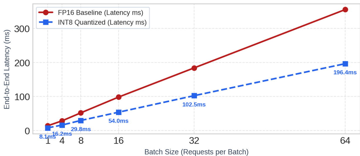
Figure 2: End-to-end inference latency comparing FP16 baseline against INT8 quantized engine.
