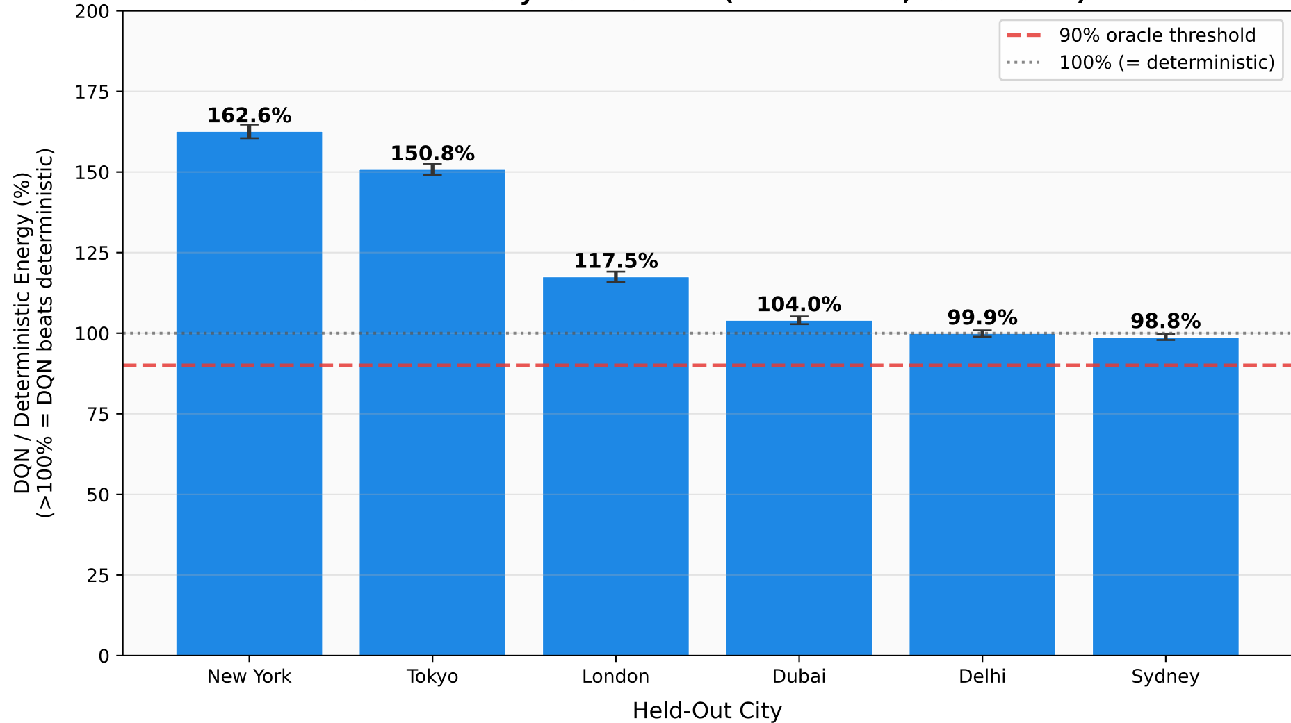
Leave-One-City-Out Transfer (Trained on 5, Tested on 1)
