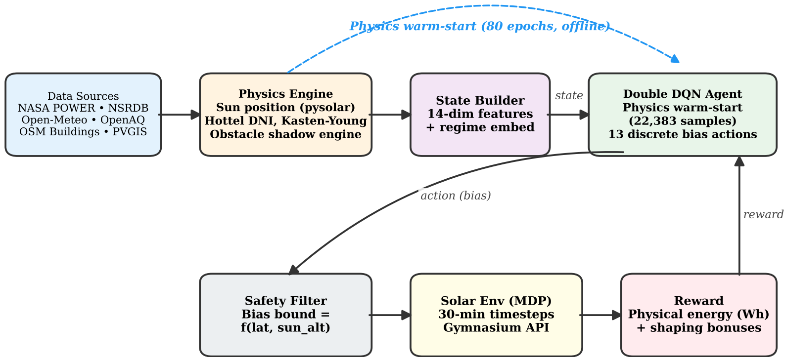
Fig. 1: Helios-X v2 — Physics-Informed RL Solar Tracking Pipeline
