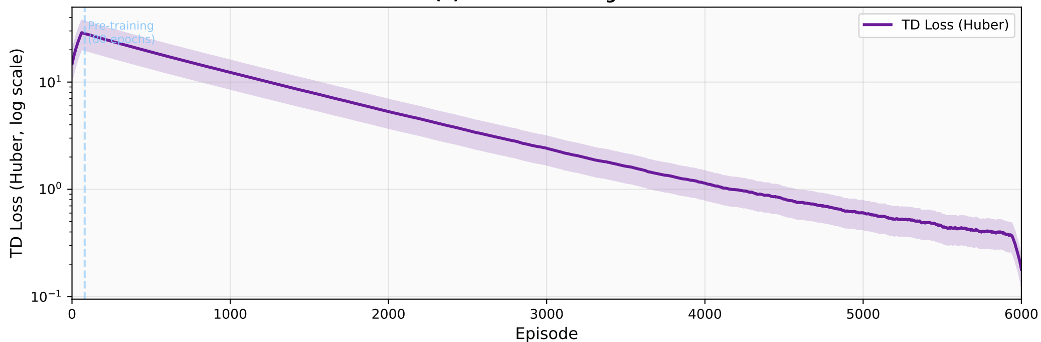
(b) TD Loss Convergence
