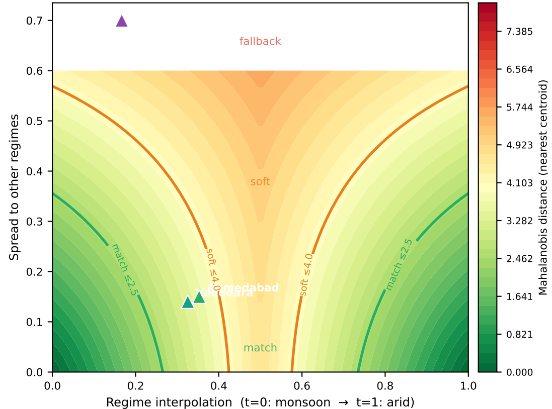
B — Mahalanobis Decision Landscape
