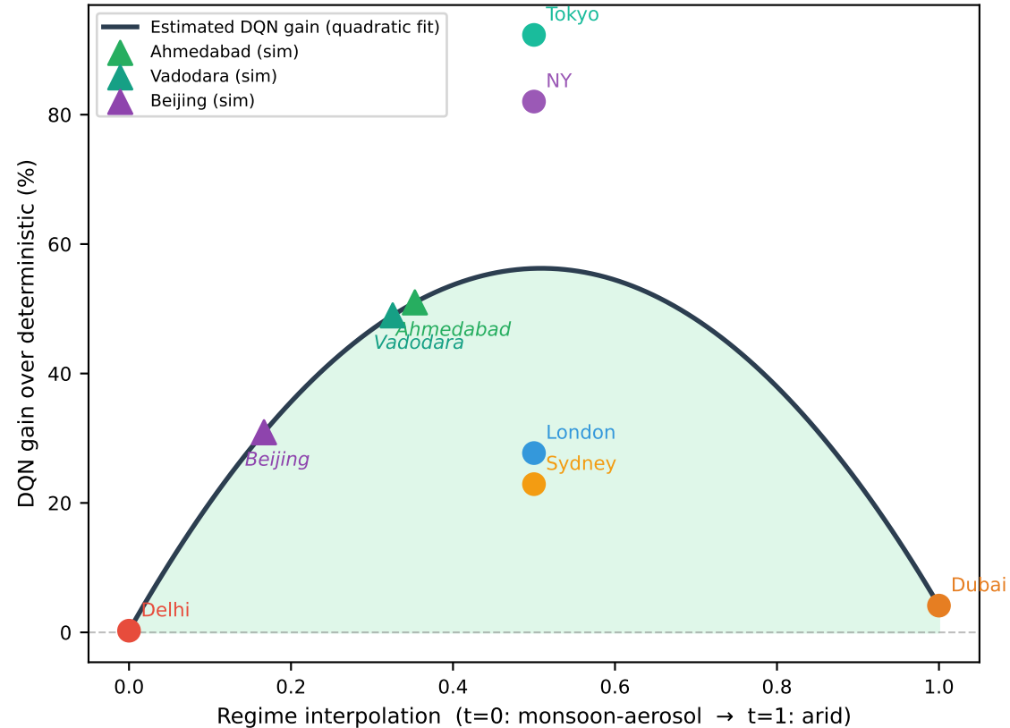
A — DQN Gain vs Regime Axis
