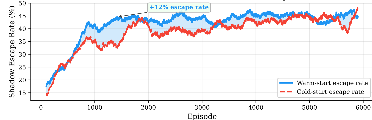
(c) Shadow Avoidance — Warm-Start Learns Escape Earlier
