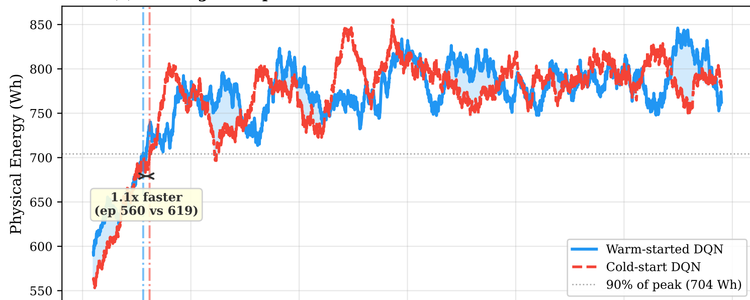
(a) Convergence Speed — Warm-Start Reaches 90% Performance Faster
