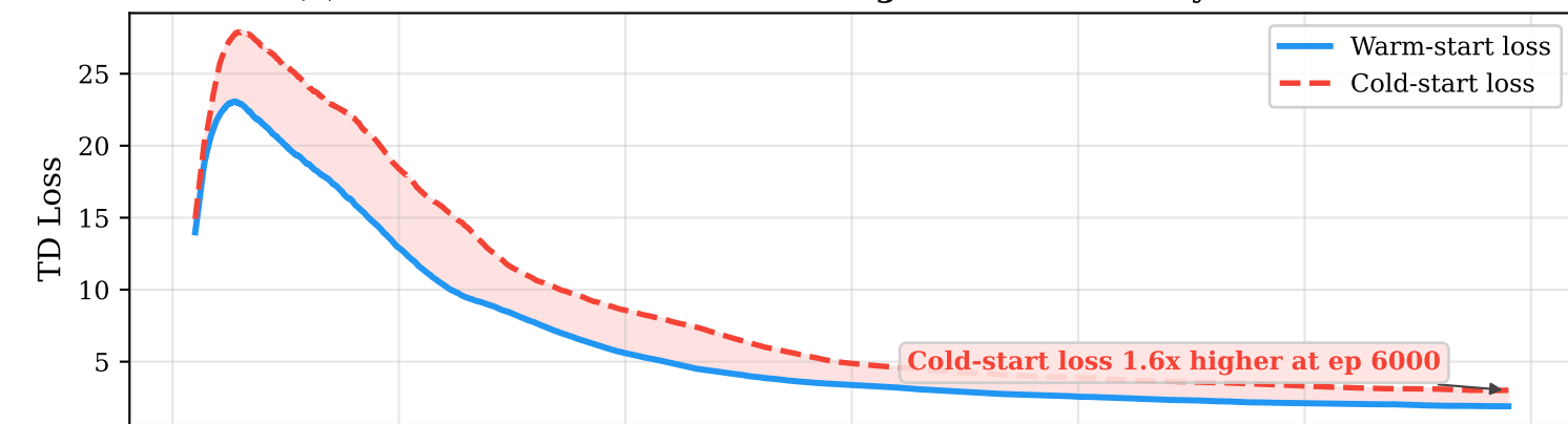
(b) TD Loss — Warm-Start Converges to Permanently Lower Loss
