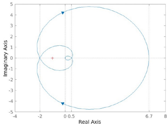
Figure 17: Nyquist plot of L(s) .
