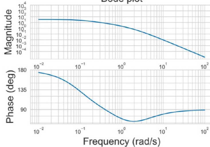
Bode plot
