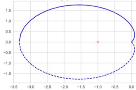
Nyquist plot 3
