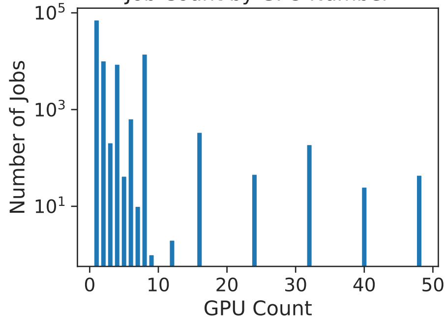
Job Count by GPU Number
