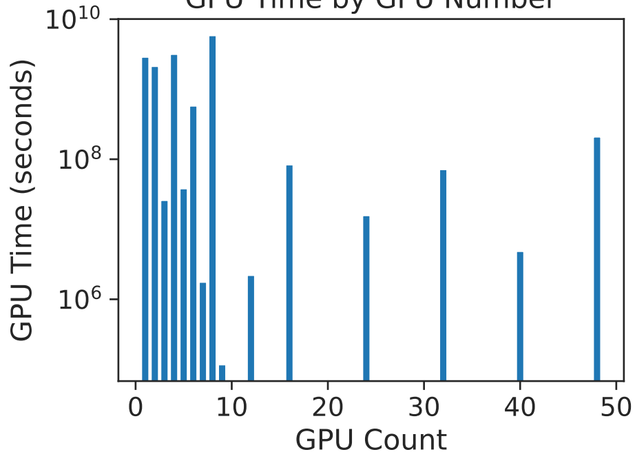
GPU Time by GPU Number
