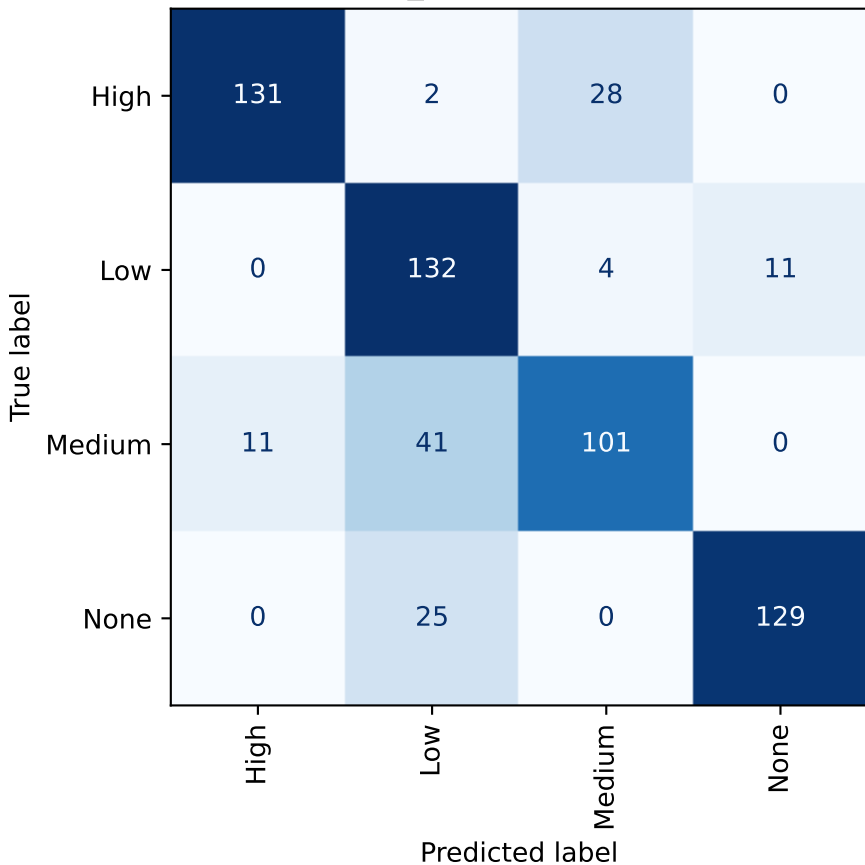
CNN — iq_imbalance (validation)
