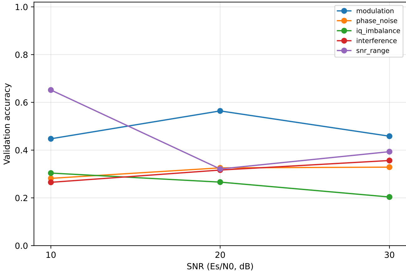
VLM accuracy vs SNR (per task)
