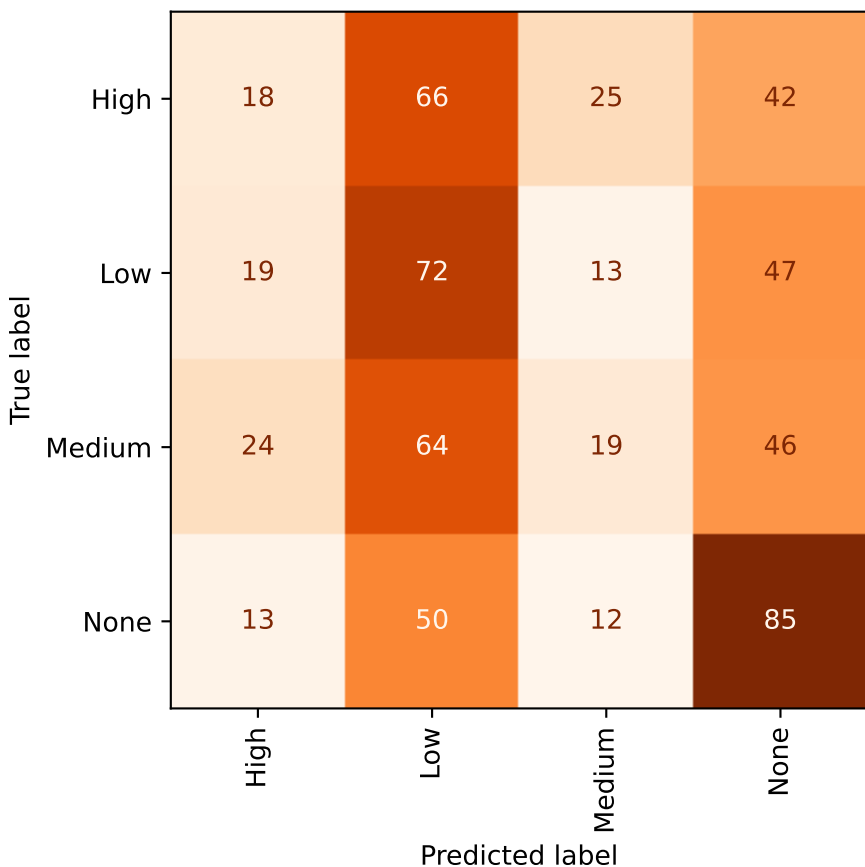
VLM — interference (validation)
