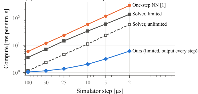
(b) Cost when solved in lockstep with the simulator
