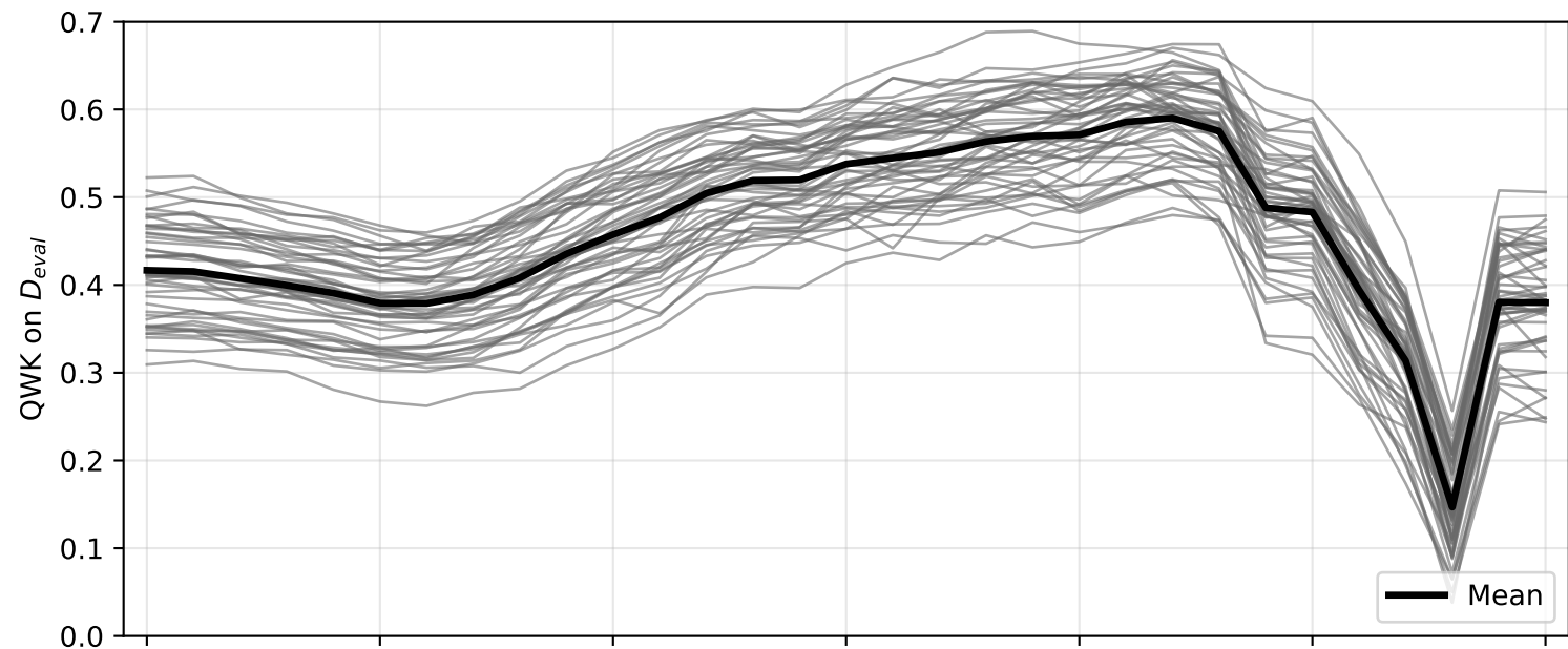
Prompt 1, Mistral-7B (n=50, |D_{sel}|=7 )
