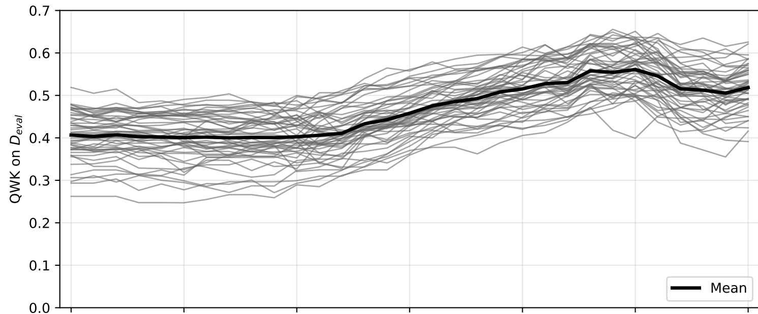
Prompt 3, Mistral-7B (n=50, |D_{sel}|=7 )
