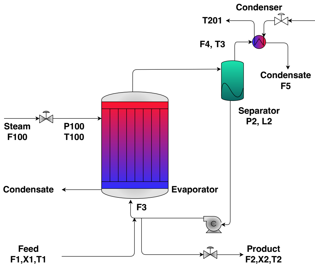
Figure 11: Schematic of evaporation process.
