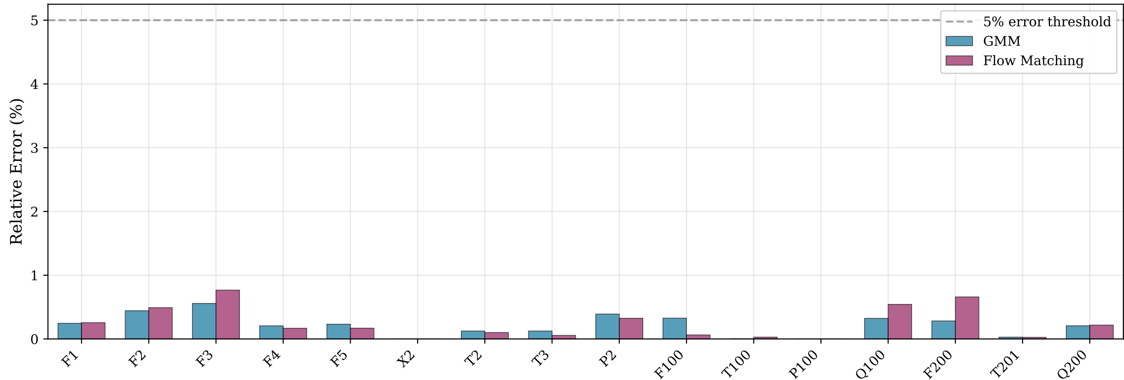
Relative Error in Decision Variables (vs. Scipy Reference)
