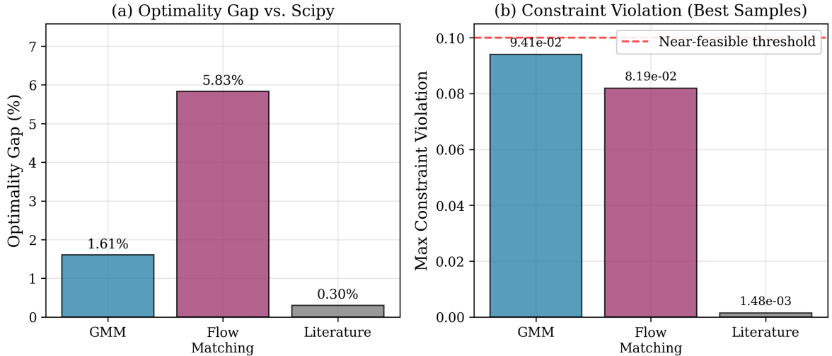
Figure 11: Summary performance comparison for the best solutions found by each generative optimization approach. (a) Optimality gap relative to the Scipy SLSQP reference solution ( -582.23 $/h). Both GMM and Flow Matching achieve small optimality gaps comparable to the literature solution. (b) Maximum equality constraint violation for the best sample from each method. The selected solutions are near-feasible with constraint violations below the 0.1 threshold, demonstrating that conditioning on X_2 = 35.5\% , P_{100} = 400 kPa, and \mathbf{h}(\mathbf{x}) = \mathbf{0} effectively guides the models toward the feasible region.
