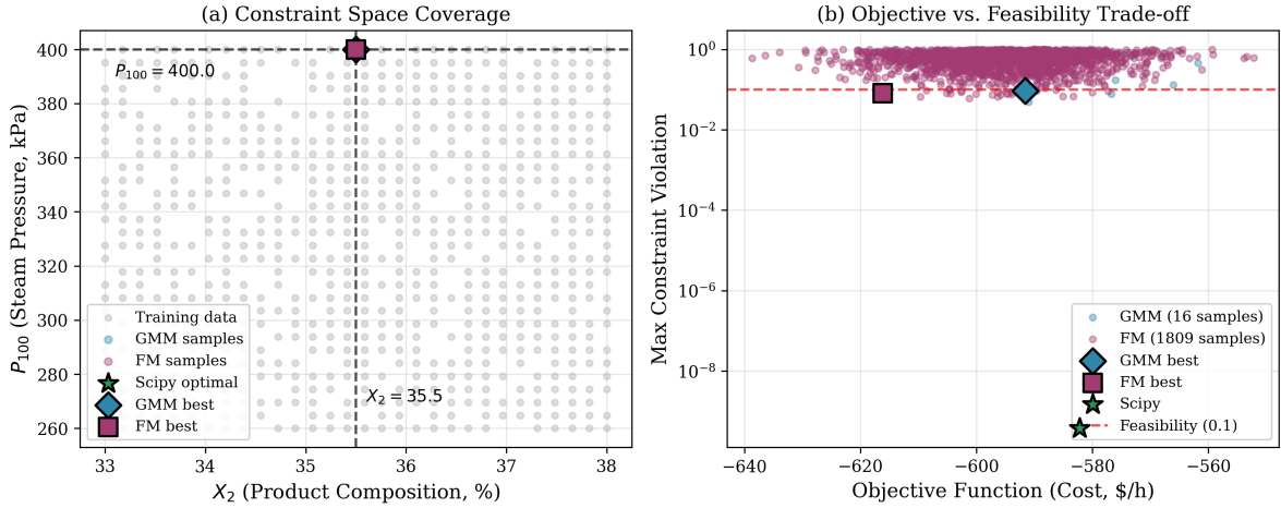
Figure 9: Training data coverage and generative model sampling for the evaporator optimization problem. (a) Constraint space showing the diverse training data generated via constraint variation ( X_2^{\min} \in [33, 38]\% , P_{100}^{\max} \in [260, 400] kPa), along with samples generated by GMM and Flow Matching when conditioned on the target values X_2 = 35.5\% and P_{100} = 400 kPa. The GMM samples cluster tightly at the conditioned values, while Flow Matching samples show slight spread around the target. (b) Trade-off between objective function value and constraint satisfaction. Both methods generate samples near the Scipy optimal solution, with Flow Matching producing more samples in the near-feasible region (violation < 0.1 ).
