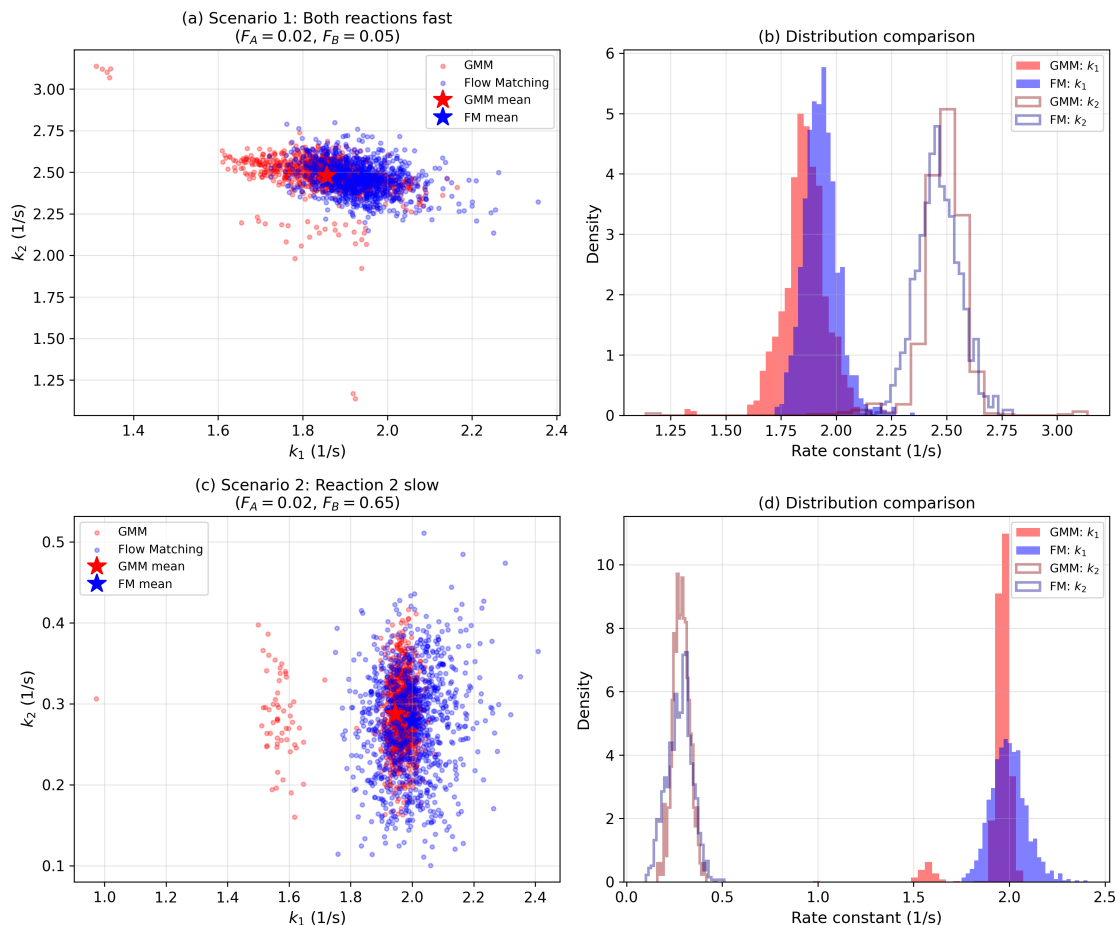
Figure 13: Estimating rate constants ( k_1, k_2 ) from reactor exit flows ( F_A, F_B ) using GMM and Flow Matching. Left panels show joint distributions in parameter space; right panels show marginal distributions. (a-b) Scenario 1 ( F_A = 0.02, F_B = 0.05 ): Both reactions fast, requiring high k_1 and k_2 . (c-d) Scenario 2 ( F_A = 0.02, F_B = 0.65 ): First reaction fast, second slow, requiring high k_1 and low k_2 . Both methods correctly identify the parameter regimes. GMM shows minor multimodality due to the non-unique inverse problem, while Flow Matching produces smoother distributions. Mean estimates (stars) accurately reproduce the target observations.
