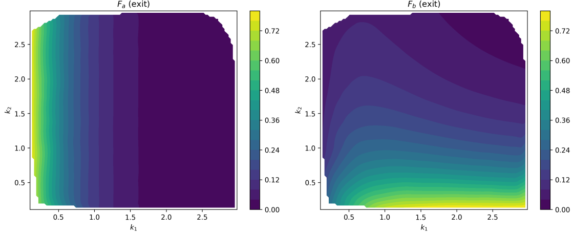
Figure 12: Contour plots of the relationships between k_1 and k_2 and a) F_A and b) F_B .
