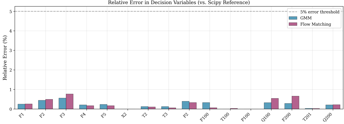
Figure 10: Relative error in each decision variable for the best GMM and Flow Matching solutions compared to the Scipy reference. Most variables achieve errors below the 5% threshold (dashed line). The conditioning variables X_2 and P_{100} show near-zero error for GMM (since they are directly conditioned) and very small error for Flow Matching. Larger relative errors in some flow rates and duties reflect the sensitivity of these variables to small perturbations in the coupled system of equations.
