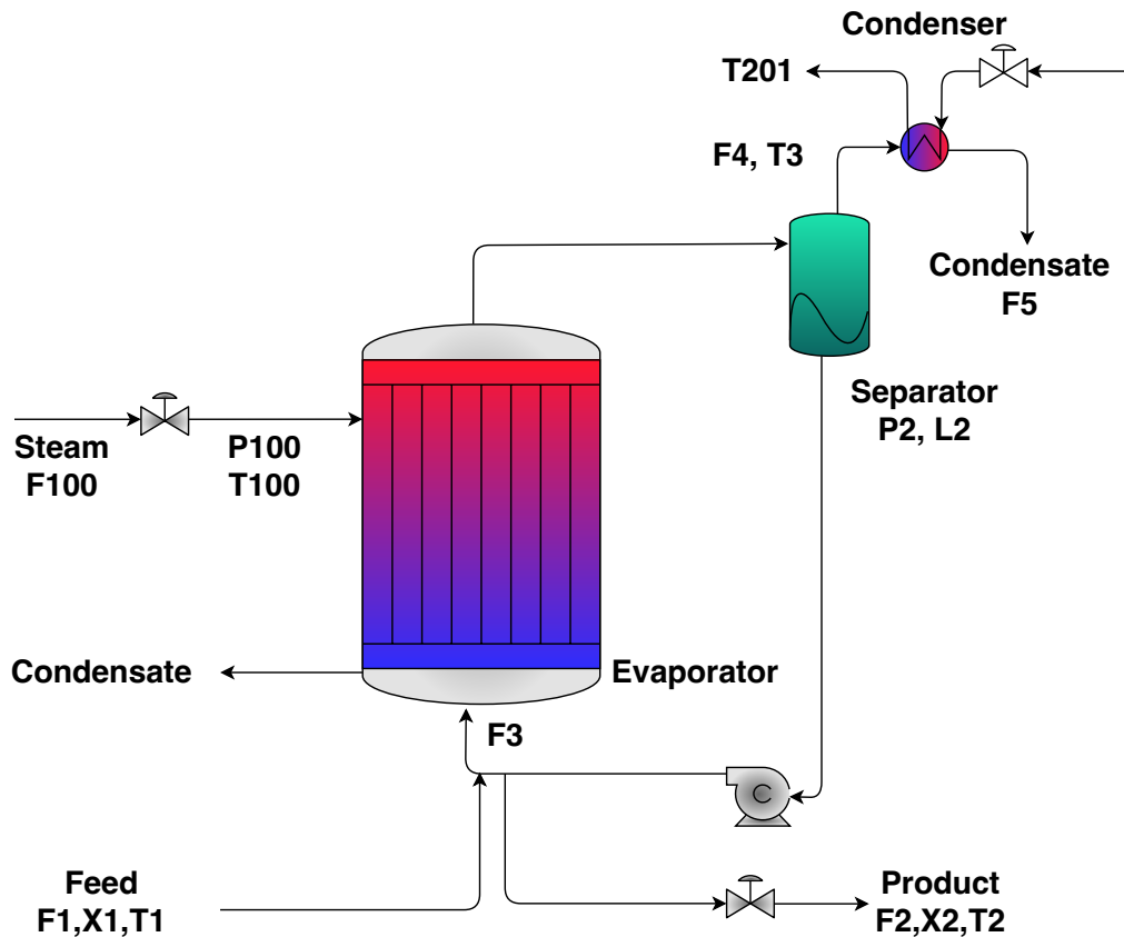
Figure 8: Schematic of evaporation process.
