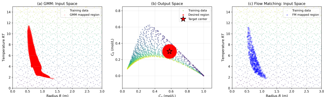
Figure 11: Mapping a desired concentration region (b, red circle: C_a = 0.58 , C_b = 0.30 \pm 0.08 mol/L) to feasible design parameters using (a) GMM and (c) Flow Matching. Both methods identify the irregular, non-convex region in (R, RT) space that produces the target concentrations. Background points show training data colored by distance from origin. The complex shape of the mapped region reveals the nonlinear relationship between reactor size, temperature, and exit concentrations, demonstrating that multiple design configurations can achieve the same production target. This inverse mapping capability is unique to generative models.
