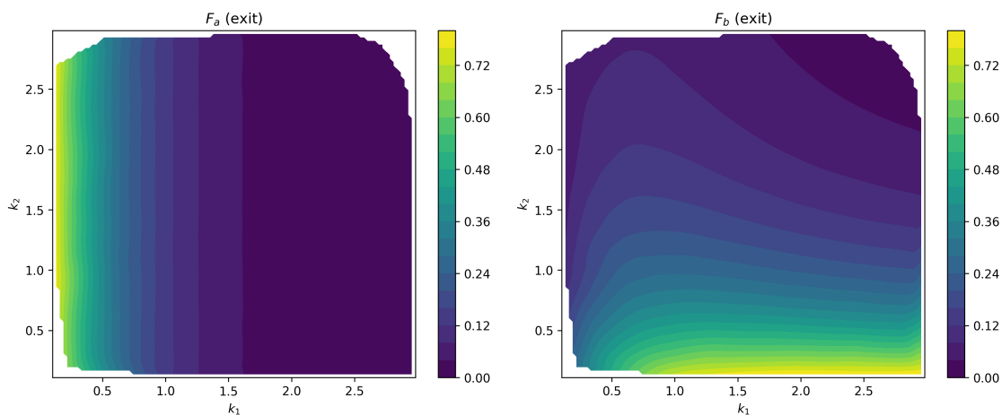
Figure 9: Contour plots of the relationships between k_1 and k_2 and a) F_A and b) F_B .
