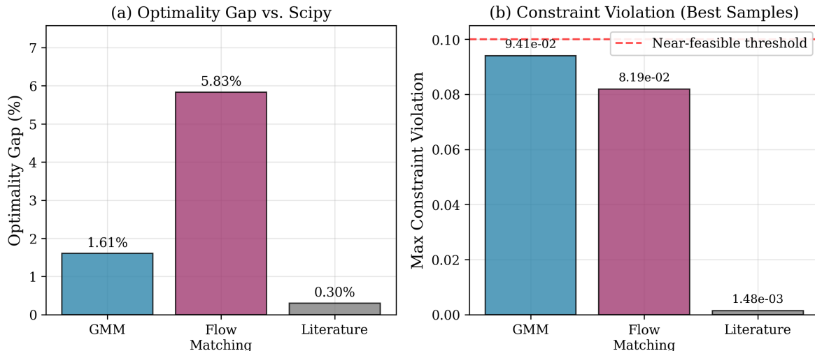
Figure 14: Summary performance comparison for the best solutions found by each generative optimization approach. (a) Optimality gap relative to the scipy SLSQP reference solution (-582.23 $/h). Both GMM and Flow Matching achieve small optimality gaps comparable to the literature solution. (b) Maximum equality constraint violation for the best sample from each method. The selected solutions are near-feasible with constraint violations below the 0.1 threshold, demonstrating that conditioning on X_2 = 35.5\% , P_{100} = 400 kPa, and \mathbf{h}(\mathbf{x}) = \mathbf{0} effectively guides the models toward the feasible region.
