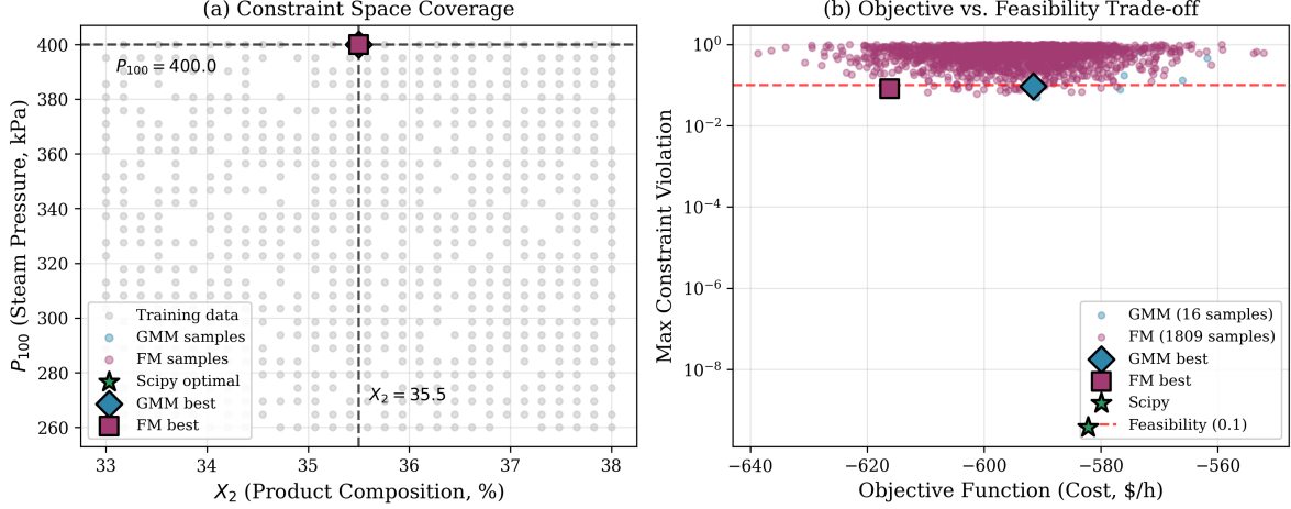
Figure 12: Training data coverage and generative model sampling for the evaporator optimization problem. (a) Constraint space showing the diverse training data generated via constraint variation ( X_2^{\min} \in [33, 38]\% , P_{100}^{\max} \in [260, 400] kPa), along with samples generated by GMM and Flow Matching when conditioned on the target values X_2 = 35.5\% and P_{100} = 400 kPa. The GMM samples cluster tightly at the conditioned values, while Flow Matching samples show slight spread around the target. (b) Trade-off between objective function value and constraint satisfaction. Both methods generate samples near the scipy optimal solution, with Flow Matching producing more samples in the near-feasible region (violation < 0.1 ).
