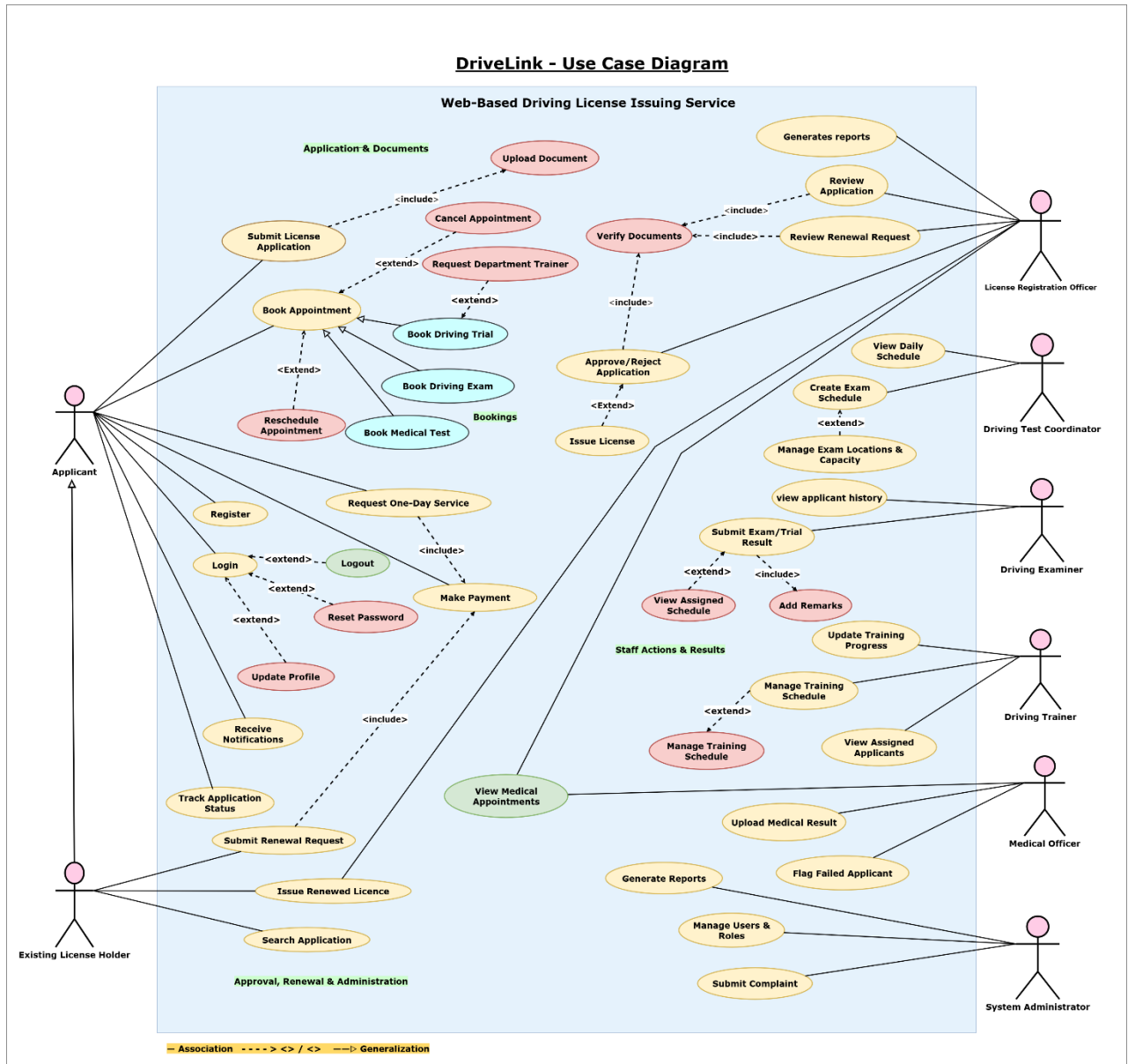
Use Case Diagram for the Web-Based Driving License Issuing Service (DriveLink)
