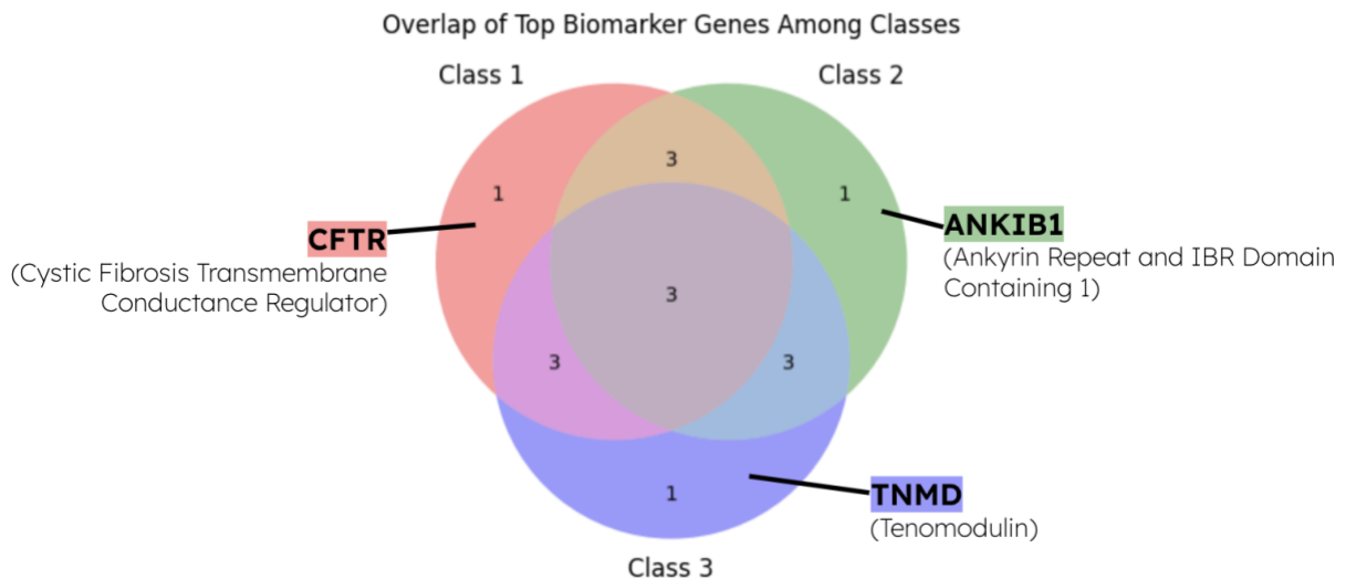
Figure 7: Venn diagram of the top 10 genes among classes; class 1=squamous cell cancer, class 2=AC unspecified, class 3=Large cell/ NOS
