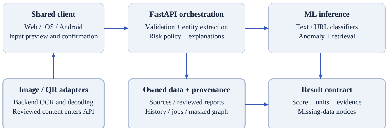
Figure 1. Prototype architecture. OCR/QR adapters normalize inputs before explicit review. Graph and retrieval context are distinct from the classifier scores. A shared result contract serves each client.
