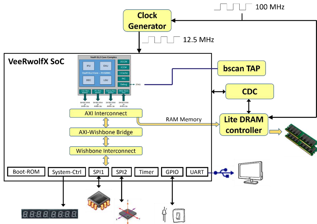
Figure 11. RVfpgaEL2-Nexys
