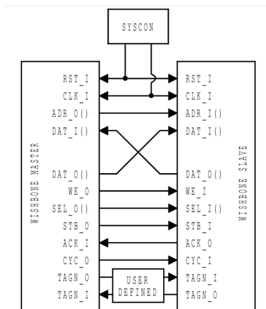
Figure 8. Wishbone Architecture
