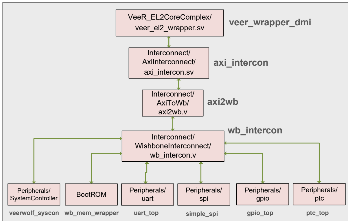
Figure 15. VeeRwolfX SoC
