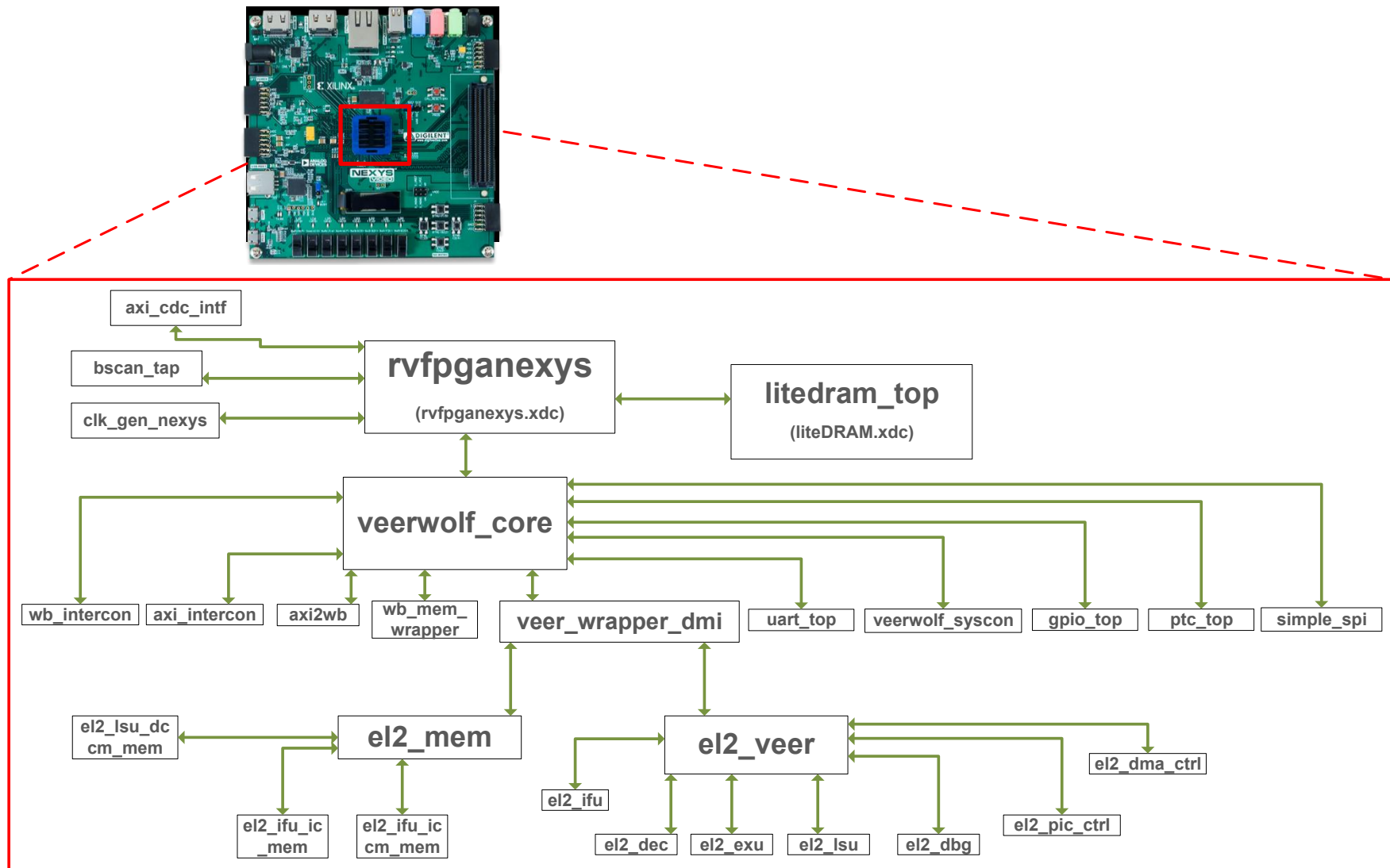
Figure 16. Modules hierarchy for the Nexys Video FPGA board implementation of RVfpgaEL2
