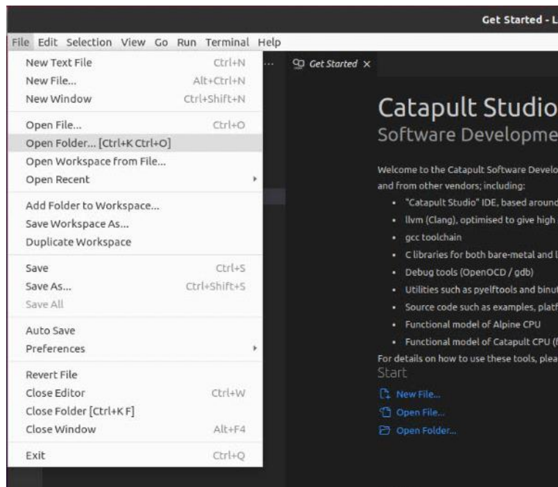
Figure 19. Open folder
