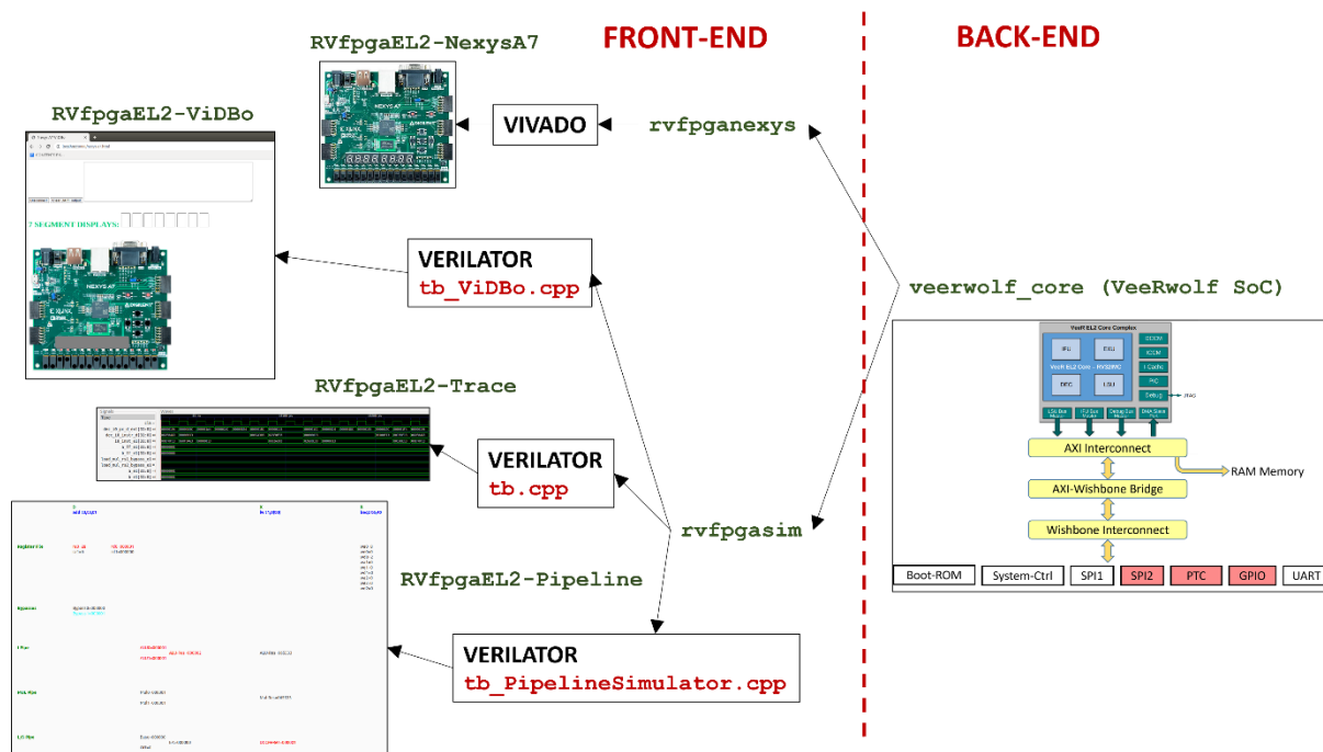
Figure 9. RVfpgaEL2 tools
