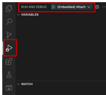
Figure 37. Start debugger
