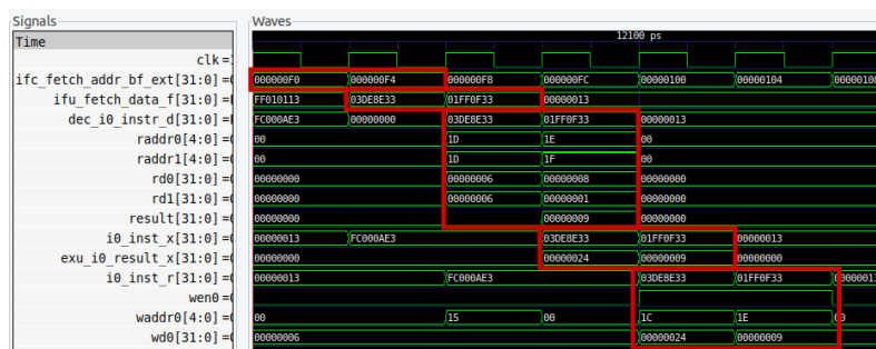
Figure 12. RVfpgaEL2-Trace
