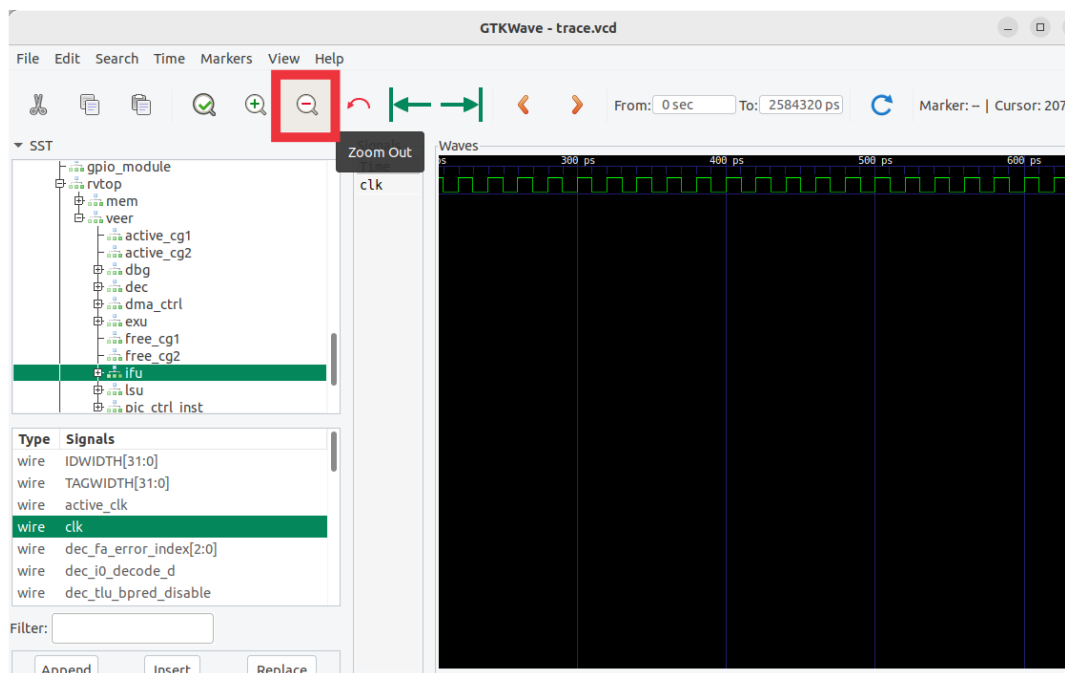
Figure 68. Zoom out
