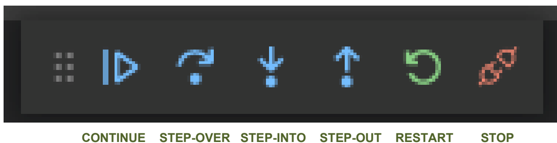
Figure 38. Debugging tools
