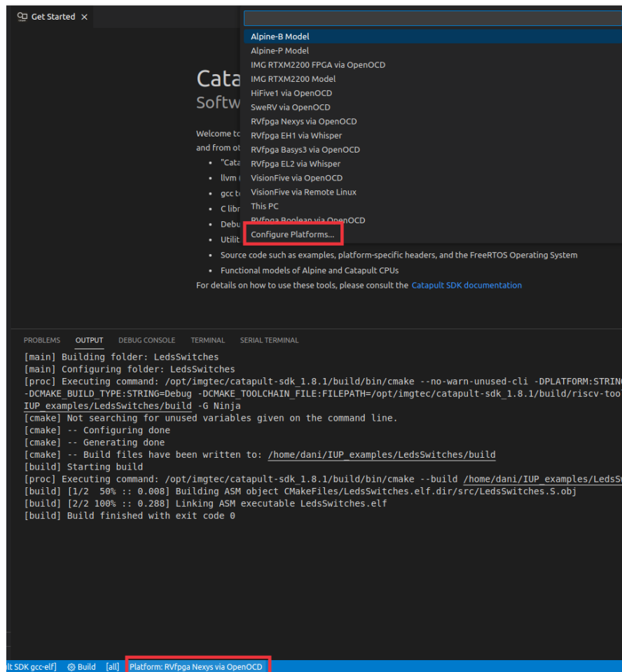
Figure 30: Configure Platforms
