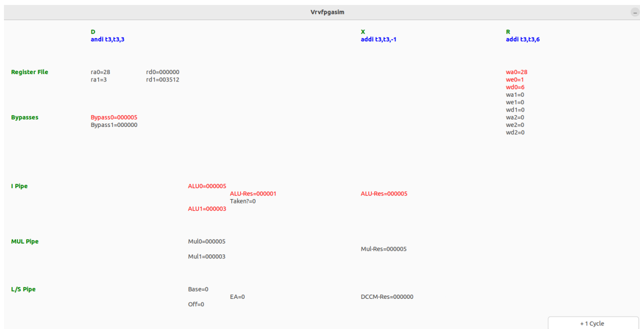
Figure 13. RVfpgaEL2-Pipeline
