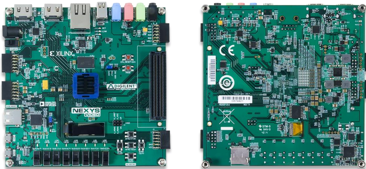
Figure 10. Digilent's Nexys Video FPGA board
