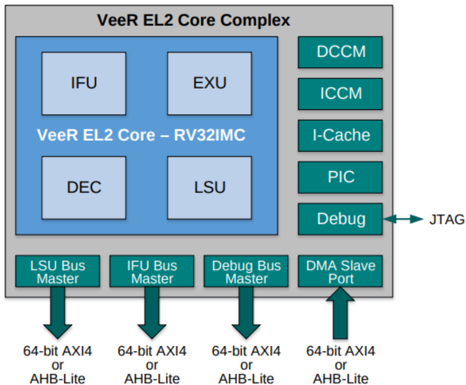
Figure 4. VeeR EL2 Core Complex
