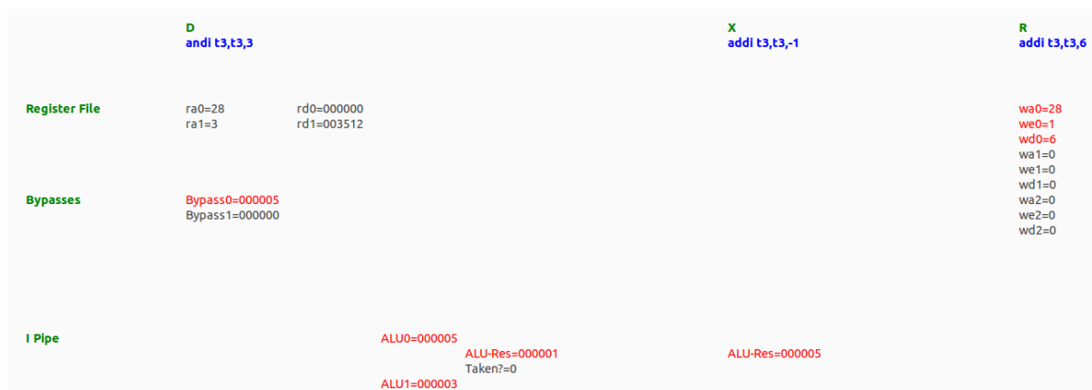
Figure 76. RVfpgaEL2-Pipeline executing AL-Operations
