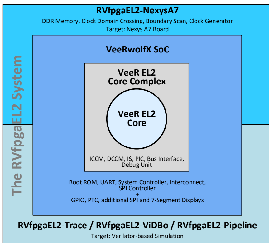
Figure 1. RVfpga System Hierarchy
