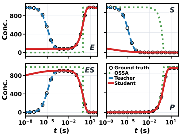
d PAKD student vs QSSA
