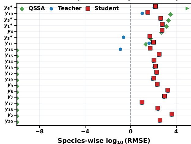
c Teacher vs Student error
