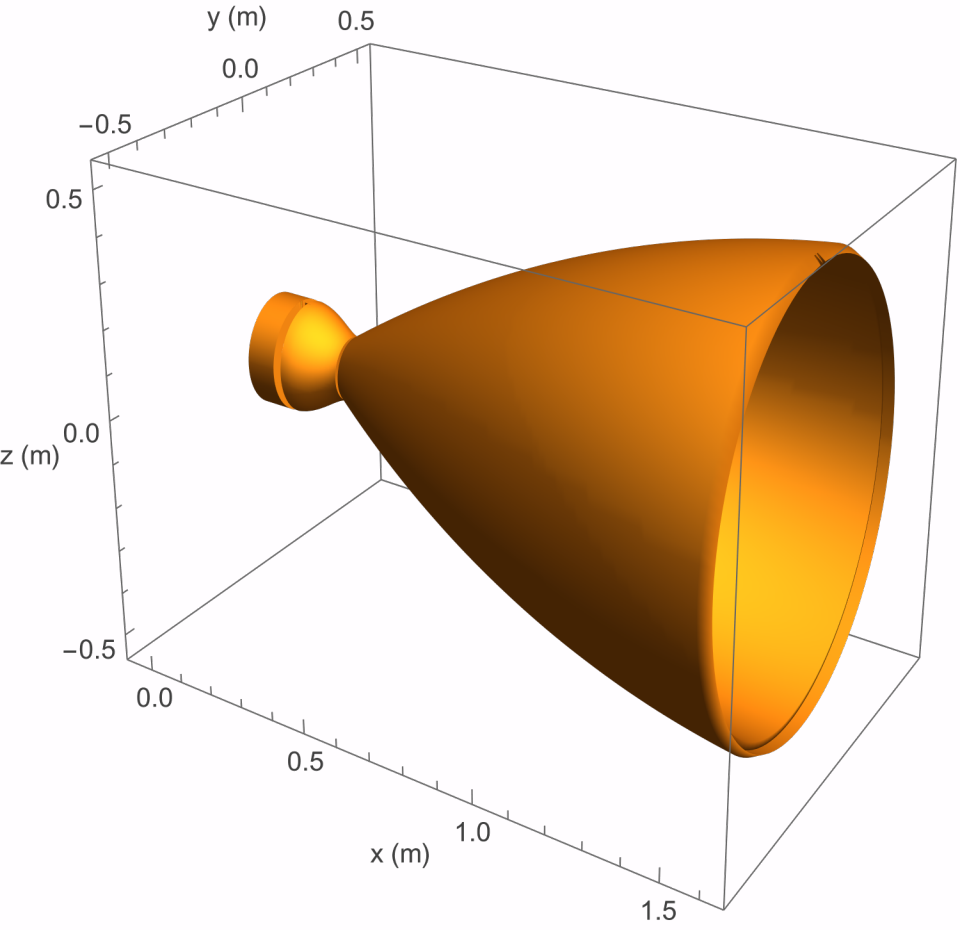
Rocket Thrust Chamber and Parabolic Bell Nozzle
