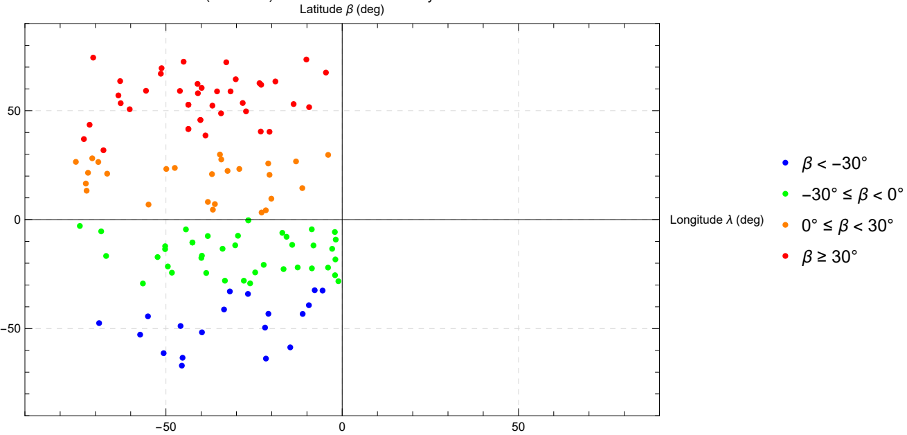
Pass 2 (Centered) – Feature Distribution by Latitude Zone
