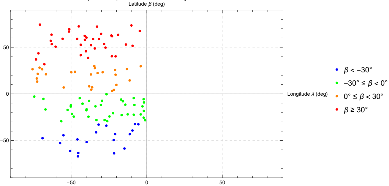
Pass 3 (Corrected) – Feature Distribution by Latitude Zone
