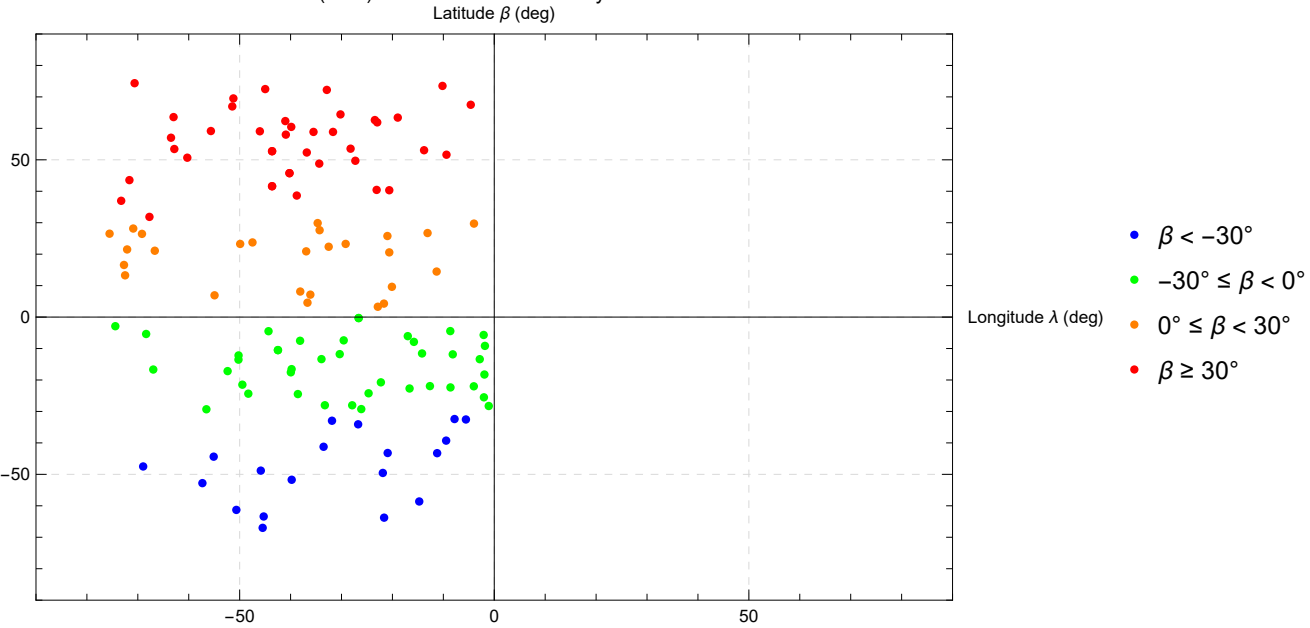
Pass 1 (Raw) – Feature Distribution by Latitude Zone
