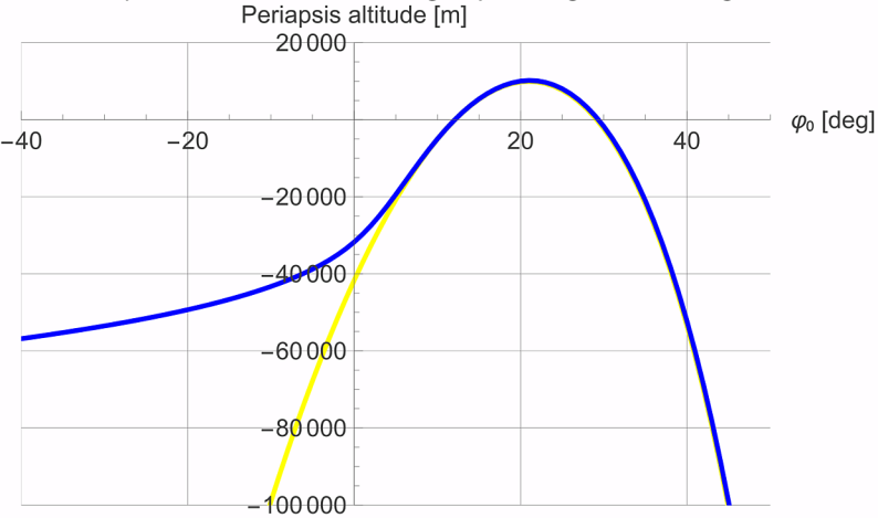
Periapsis vs Initial Thrust Angle \varphi_0 : Drag vs No Drag
