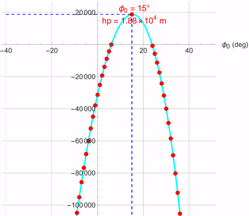
Two-Stage Rocket: Periapsis vs Initial Thrust Angle \phi_0
