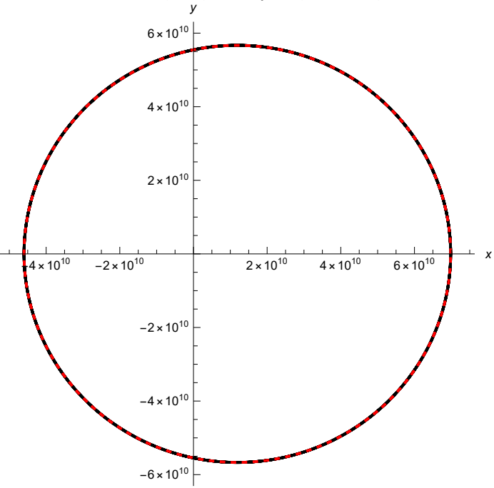
Numerical (black) vs Analytical (red dashed)
