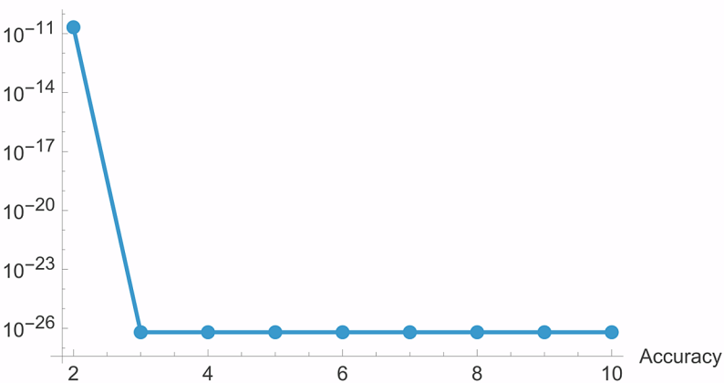
Sensitivity of Kepler Solver 'FindRoot' to Accuracy Parameters |\Delta E| (rad)
