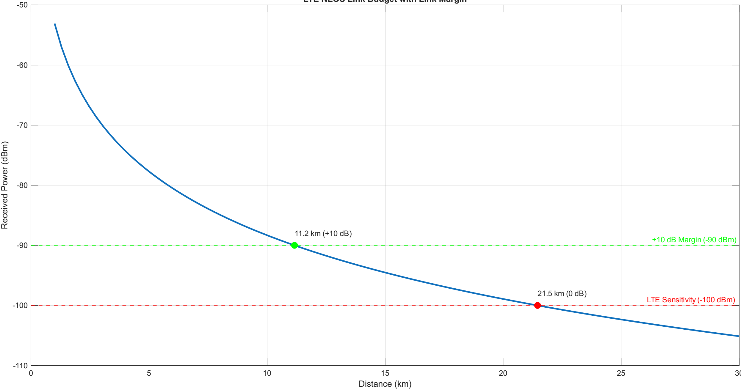
LTE NLOS Link Budget with Link Margin
