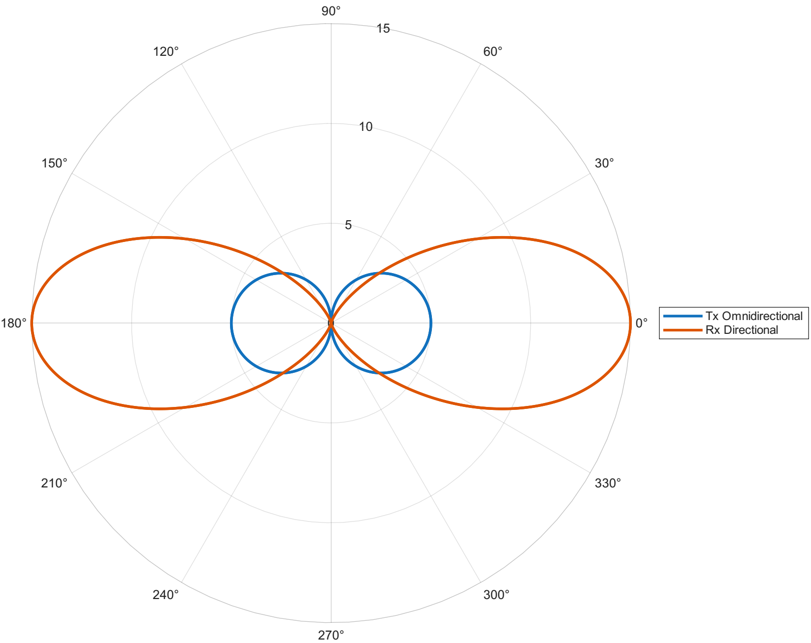
Antenna Radiation Patterns at 800 MHz
