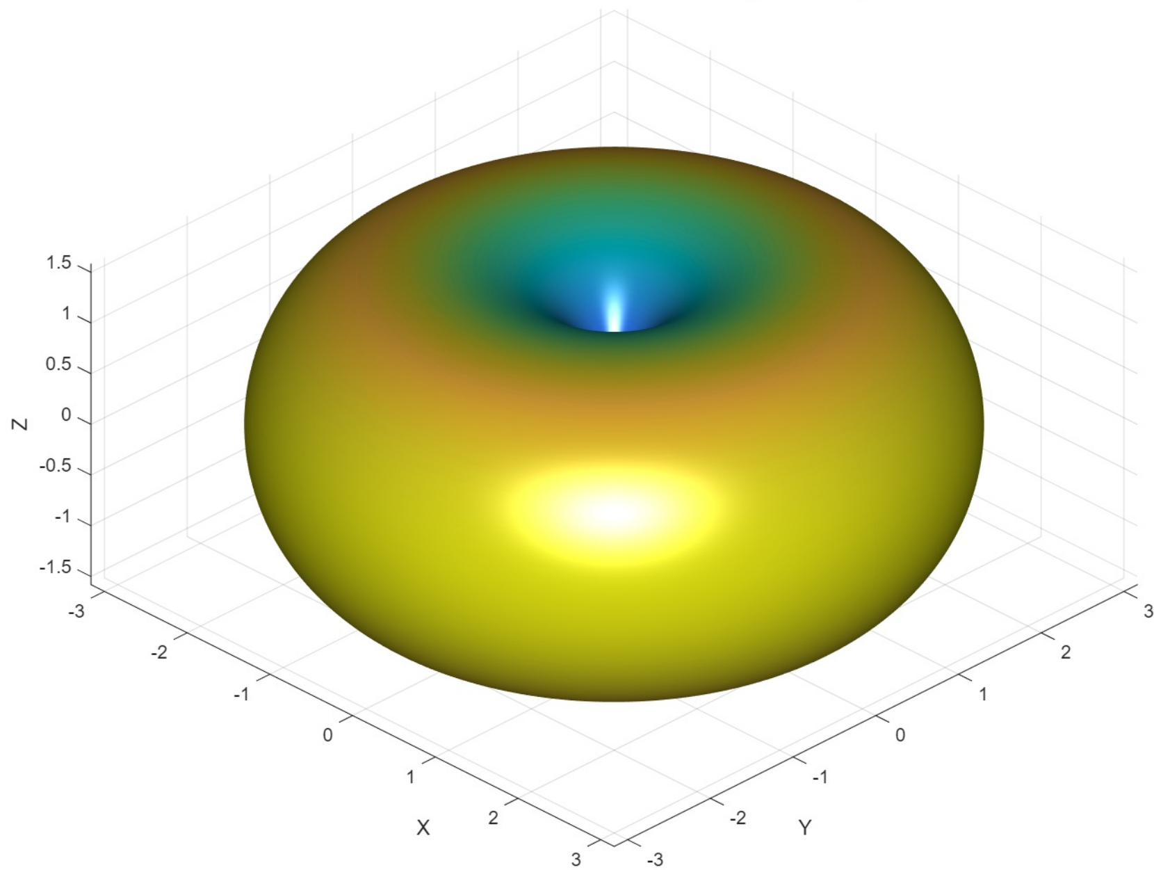
3D Transmit Antenna Radiation Pattern (Alert Node)
