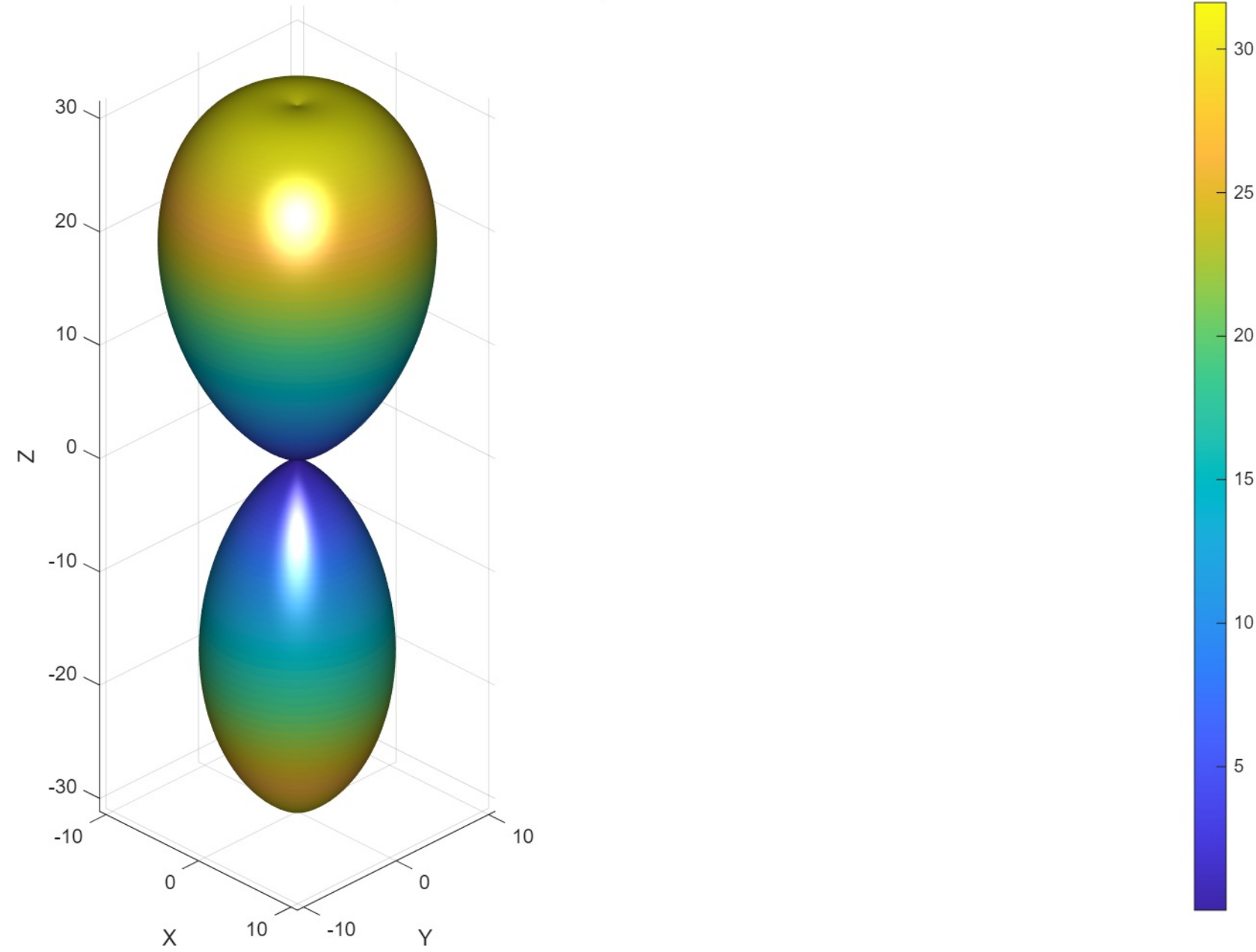
3D Receive Antenna Radiation Pattern (AFAD Base Station)
