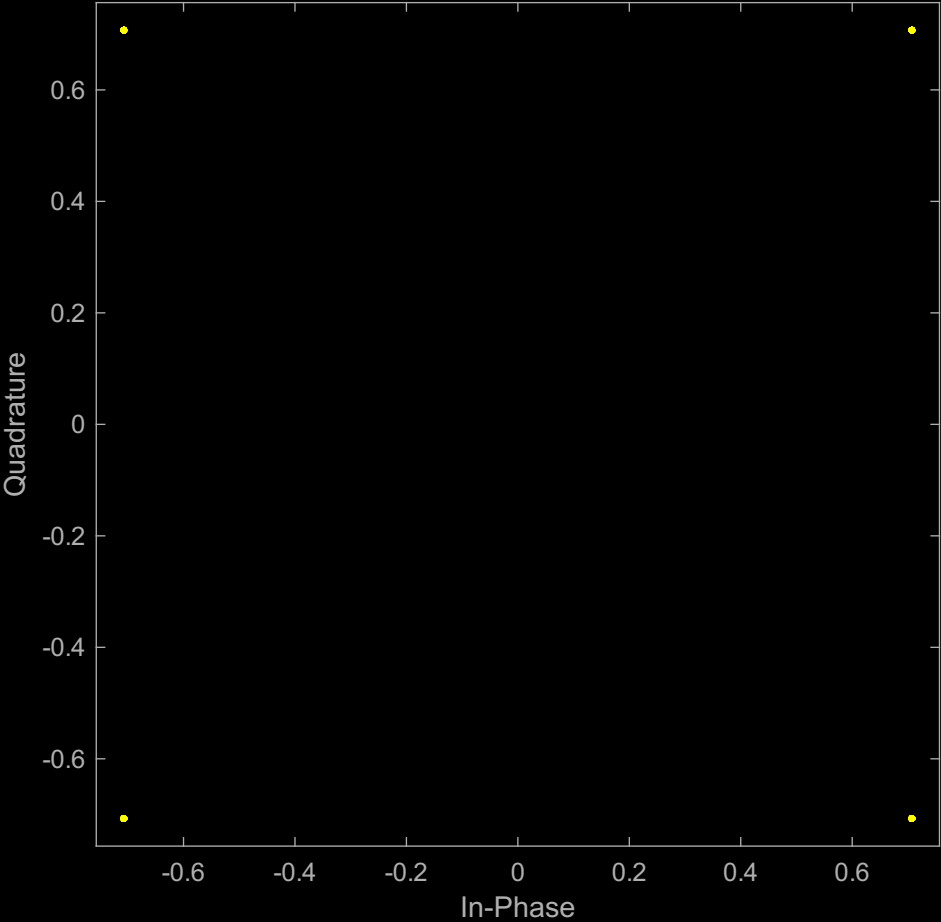
QPSK Constellation Diagram for Alert Transmission
