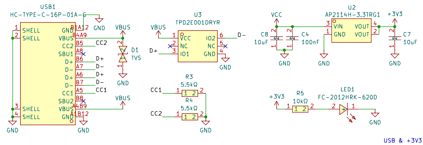
USB & +3V3
