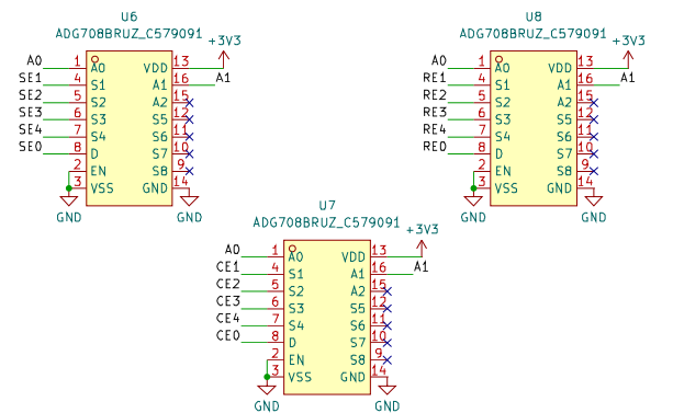
Multiplexers
