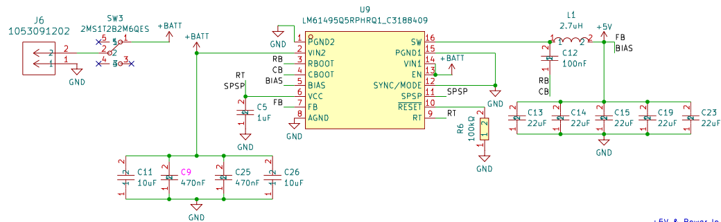
+5V & Power in
