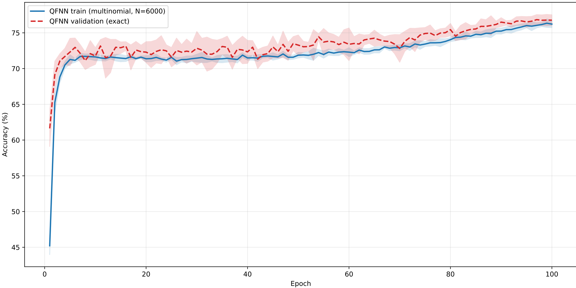
FashionMNIST8 QFNN train/validation accuracy (mean +/- sample std over 6 seeds)
