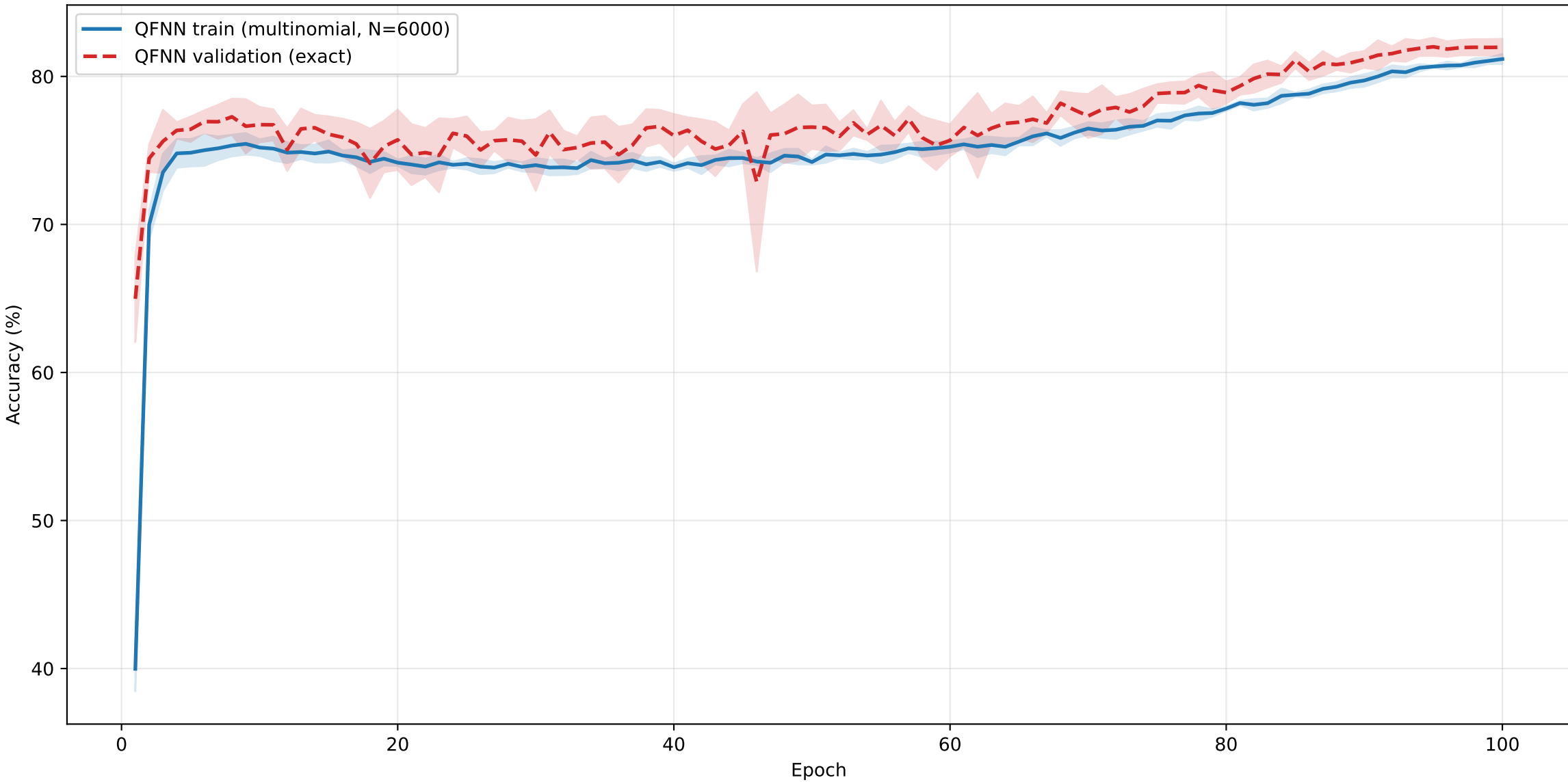
KMNIST8 QFNN train/validation accuracy (mean +/- sample std over 6 seeds)
