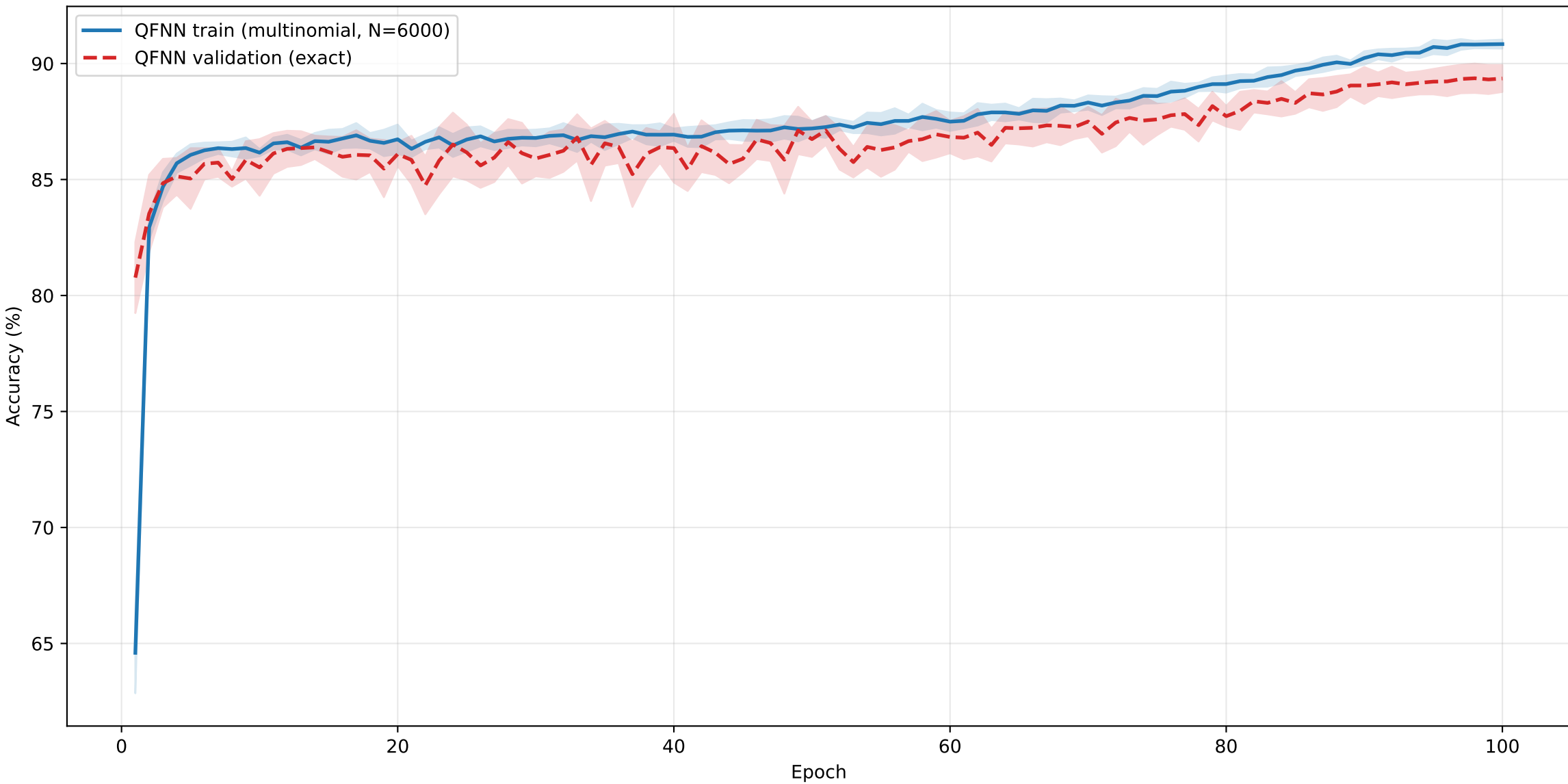
MNIST8 QFNN train/validation accuracy (mean +/- sample std over 6 seeds)
