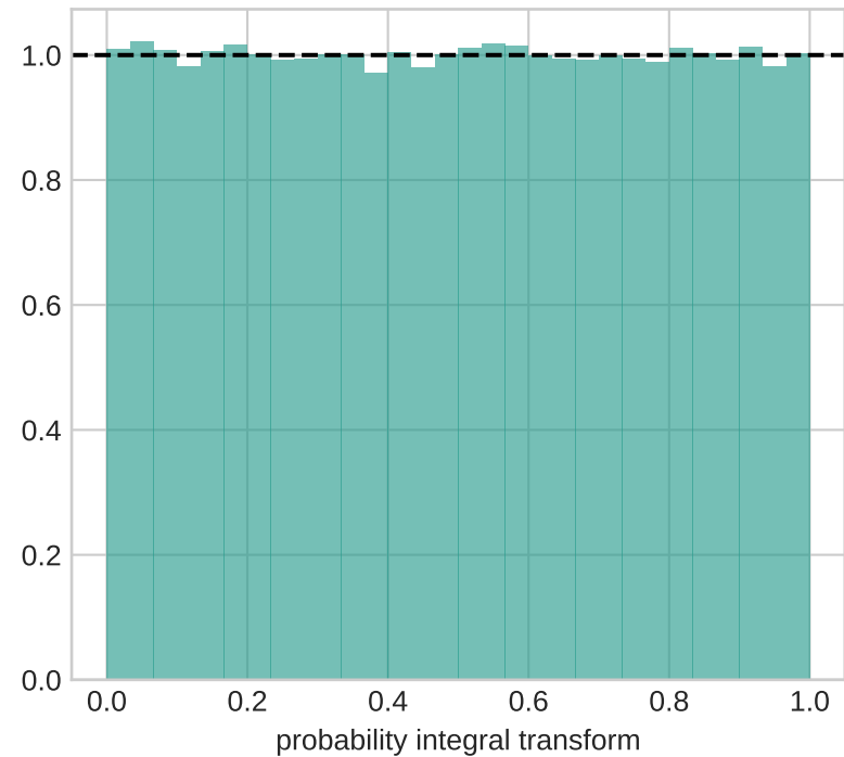
PIT: KS=0.0017
