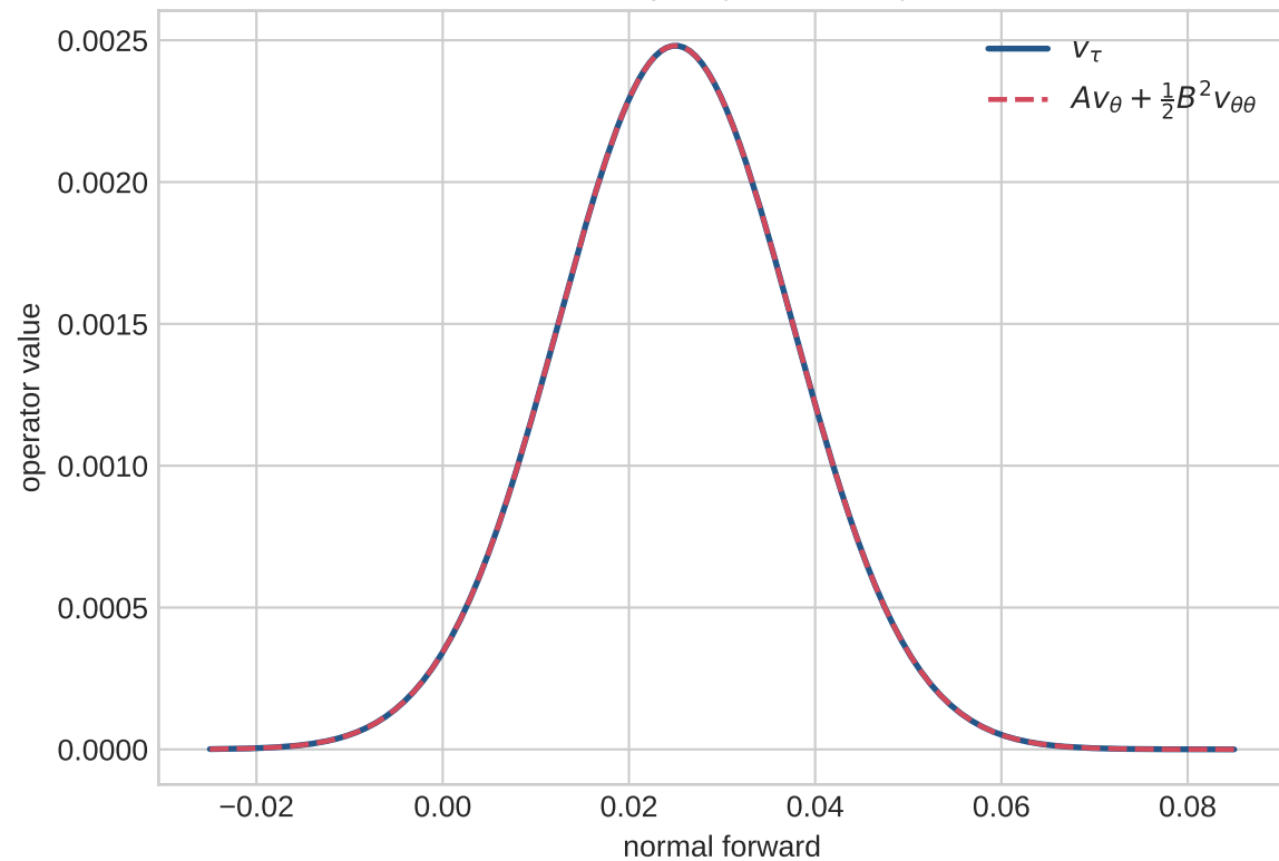
Generator equality at maturity 1.01
