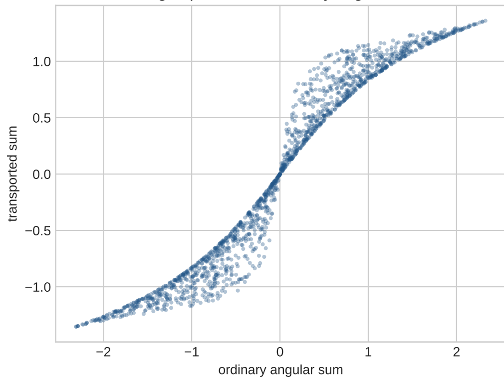
The group law is not ordinary angle addition
