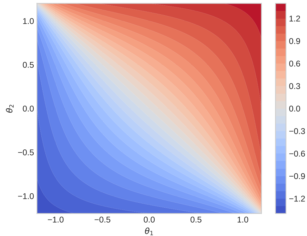
Transported sum \theta_1 \oplus \theta_2
