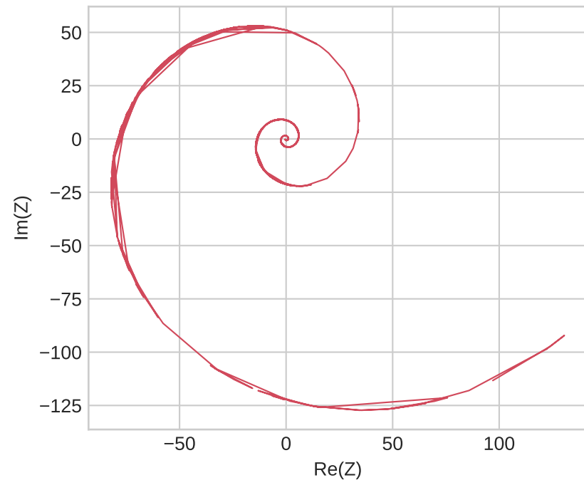
Compatible multiplicative logarithmic spiral
