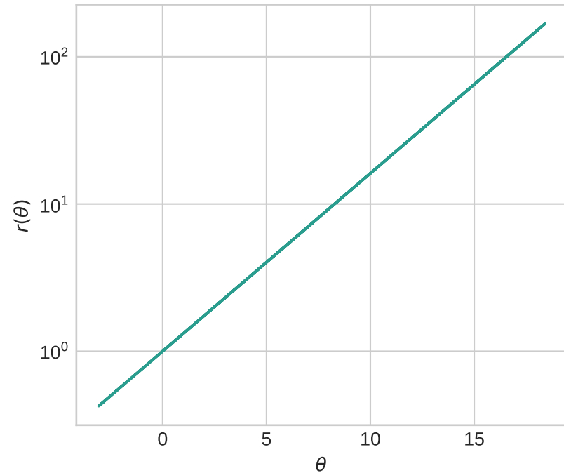
Radius encodes the winding index
